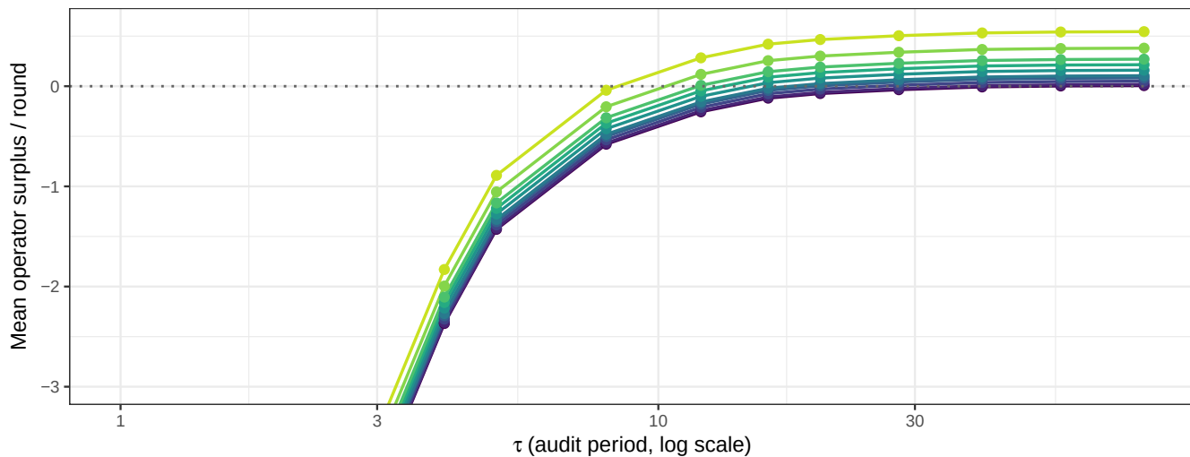
(a) Surplus near the zero-crossing, by stake (topology-invariant)
