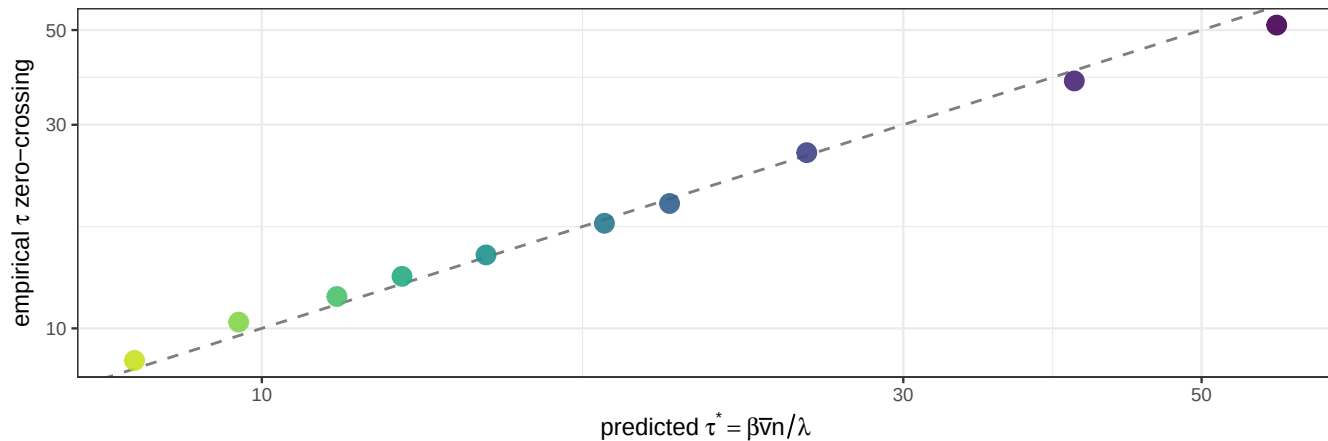
(b) SDS prediction vs empirical zero-crossing (topology-invariant)
