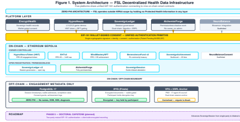
Figure 1. System architecture for sovereign behavioral health data governance.
