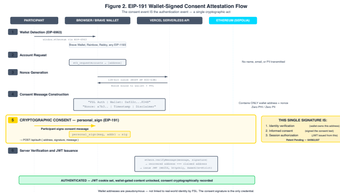
Figure 2. EIP-191 wallet-signed consent attestation flow.
