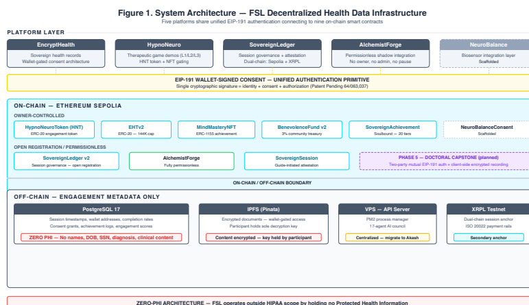
Figure 1. System architecture of the FSL decentralized health data infrastructure.
