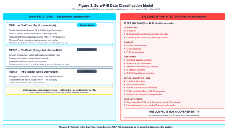
Figure 3. Zero-PHI data classification model. FSL operates outside HIPAA scope by architectural exclusion (not a covered entity, holds no PHI) — distinct from Safe Harbor de-identification, which presumes PHI existed and was stripped.
