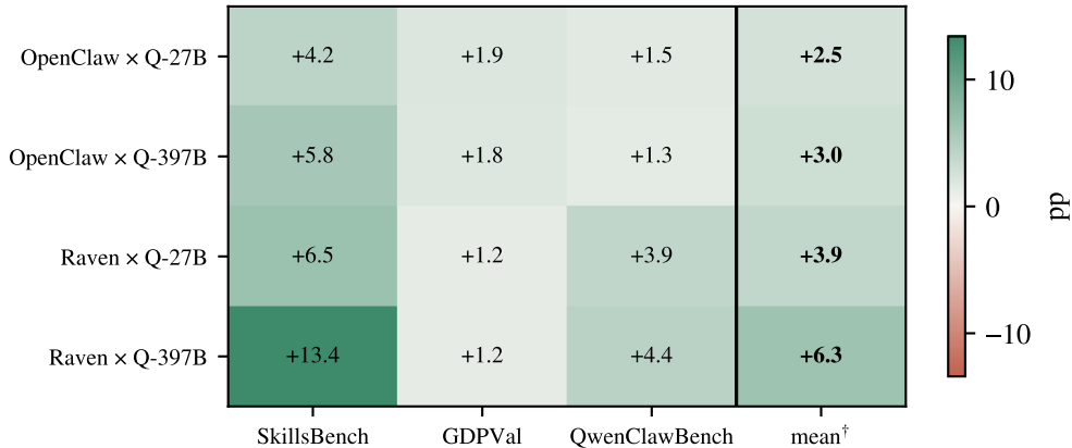
\Delta pass@1 / reward (pp), SkillCorpus vs no-skill
