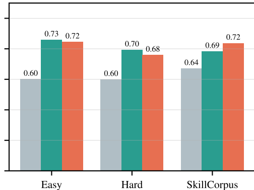
Recall@10
