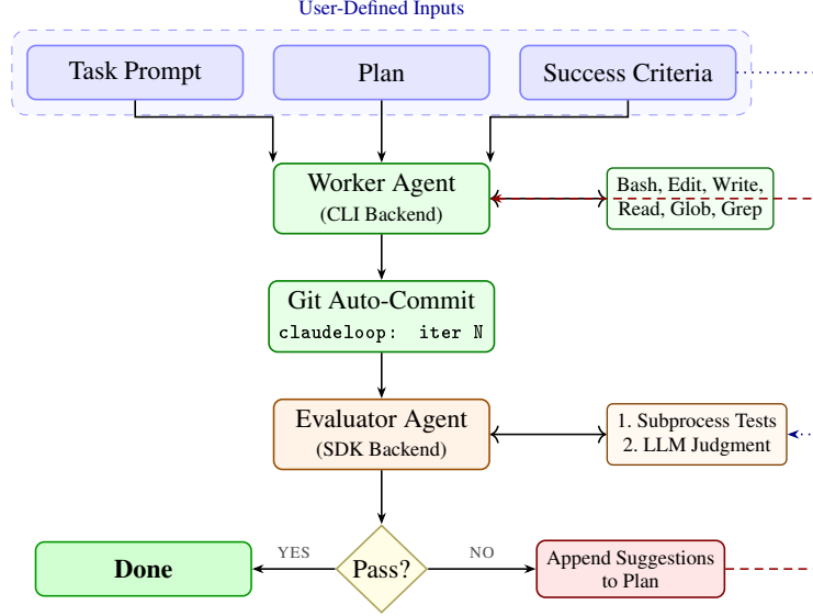
Figure 1: System overview of CLAUDELOOP. The worker implements code via Claude Code’s tools. After each iteration, changes are auto-committed and the evaluator runs deterministic tests followed by LLM judgment. On failure, suggestions are appended to the plan for the next iteration. Dotted line: success criteria also flow to the evaluator.
