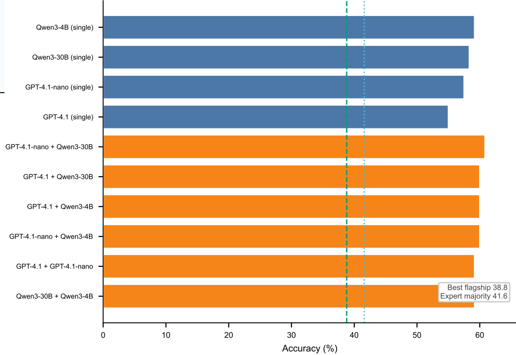
c Pairwise ensemble landscape (non-overlap detail)
