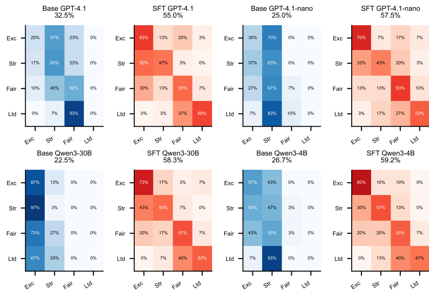
b Matched base-vs-SFT confusion maps (4 architectures)
