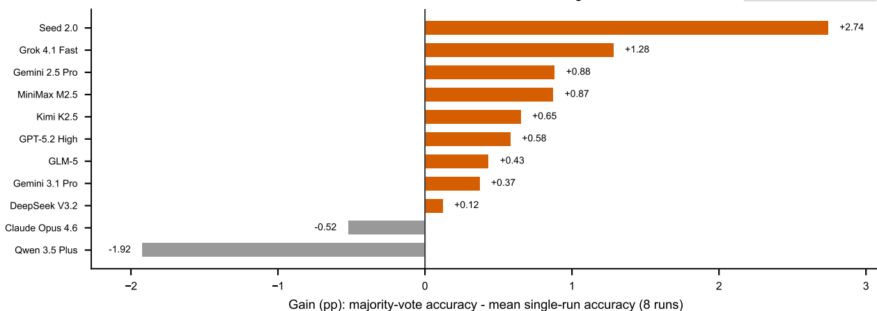
c Frontier Same-Model 8-Run Voting Gain
