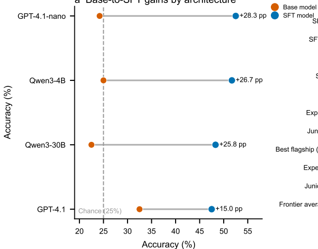
a Base-to-SFT gains by architecture
