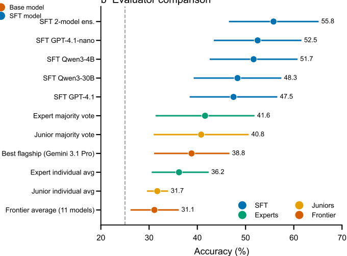
b Evaluator comparison
