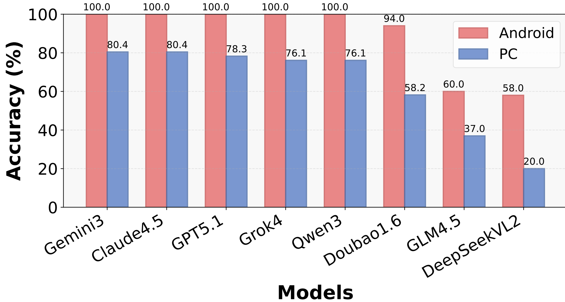
Binary Privacy Detection Accuracy
