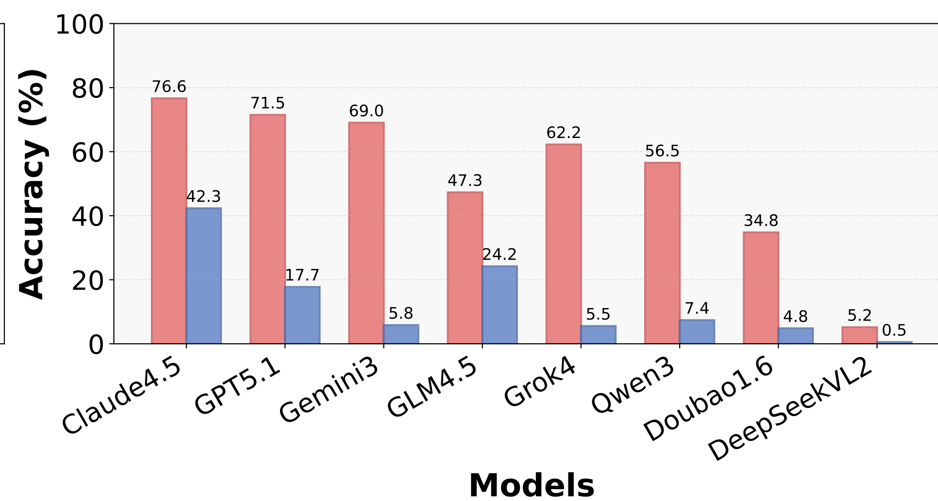
Privacy Recall Rate
