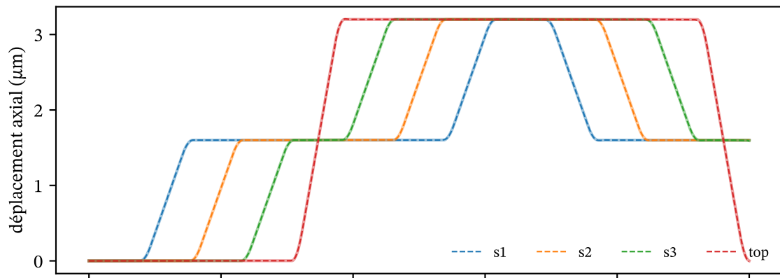
V1, fem3d, h = 1 mm : trait plein exact, tirets rockim
