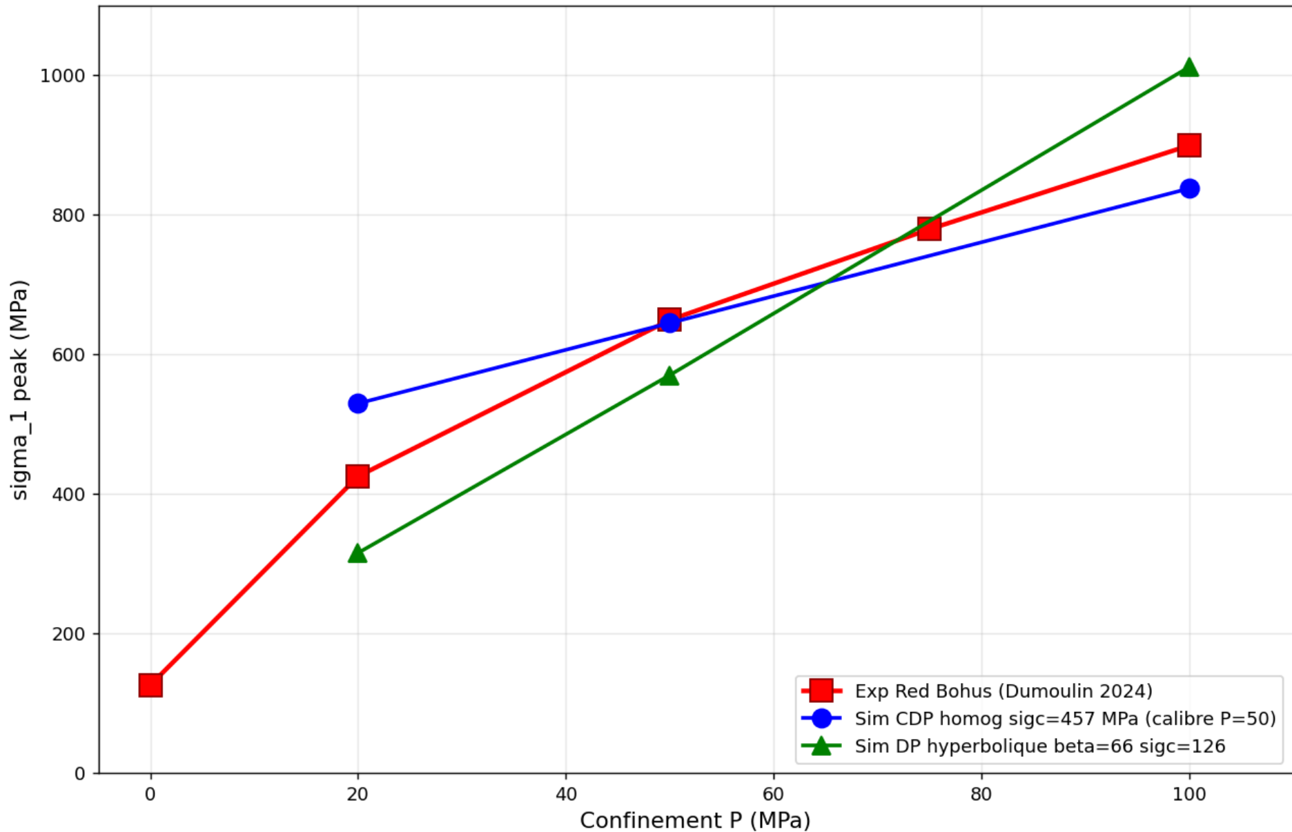
Enveloppe de rupture en compression triaxiale Comparaison sim vs experimental (Red Bohus granite)
