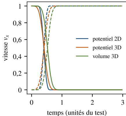
(a) choc frontal : A (trait), B (tirets)
