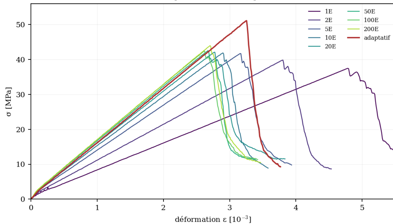
(c) compression uniaxiale (fig. 19b)
