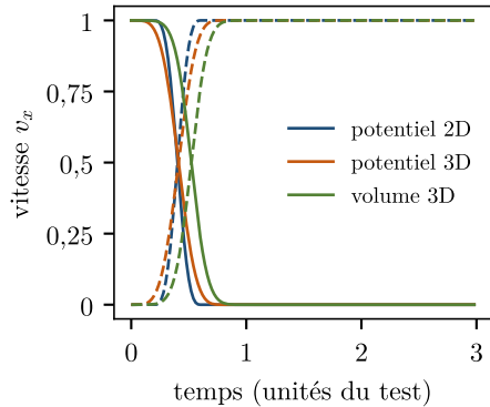
(a) choc frontal : A (trait), B (tirets)
