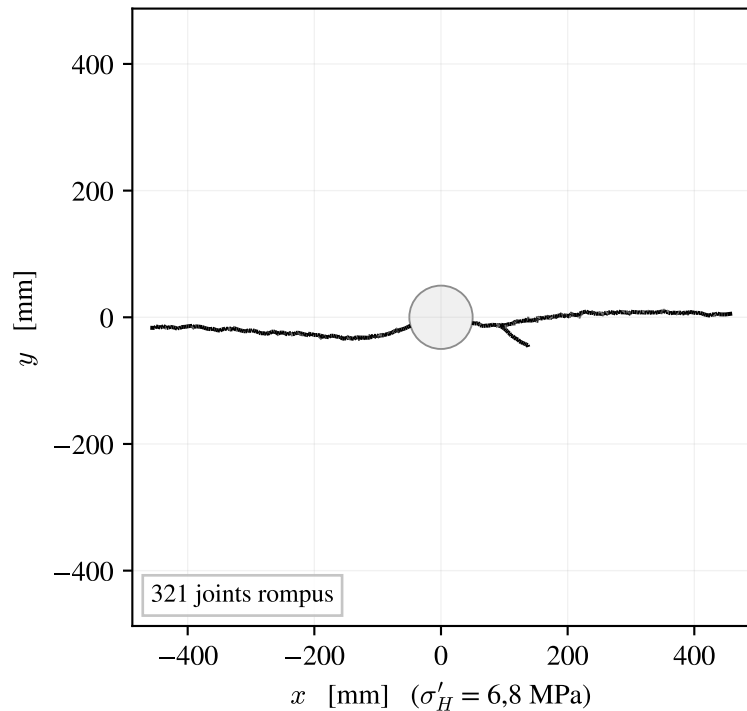
(c) Faciès anisotrope, t = 4,00 ms
