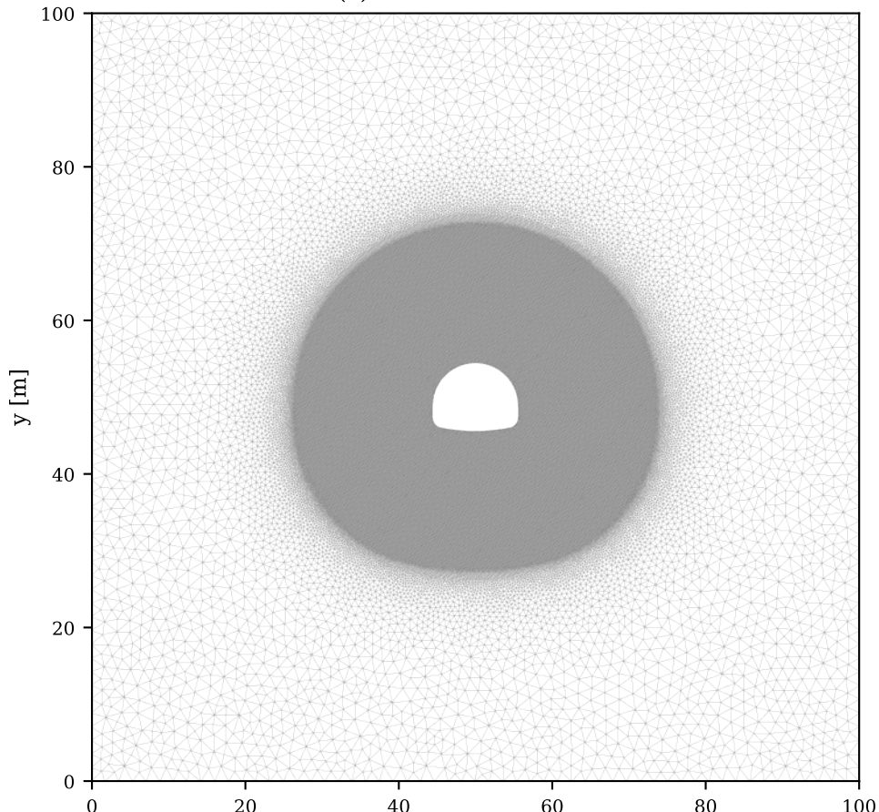
(a) modele 100 x 100 m
