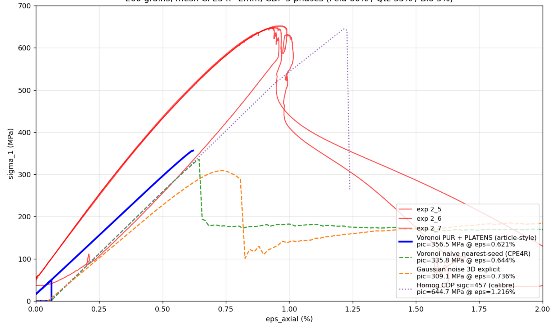
Voronoi PUR + PLATENS (article-style) - P=50 MPa, PARAM_INITIAL 200 grains, mesh CPE3 h~2mm, CDP 3 phases (Feld 60% / Qtz 35% / Bio 5%)
