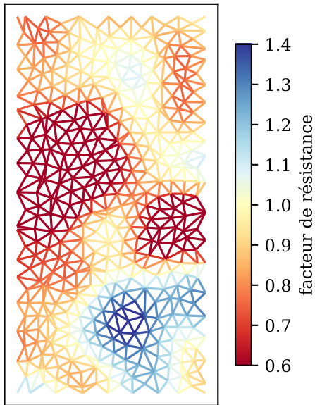
champ de Weibull corrélé ( m = 6 , \ell_{corr} = taille de grain)
