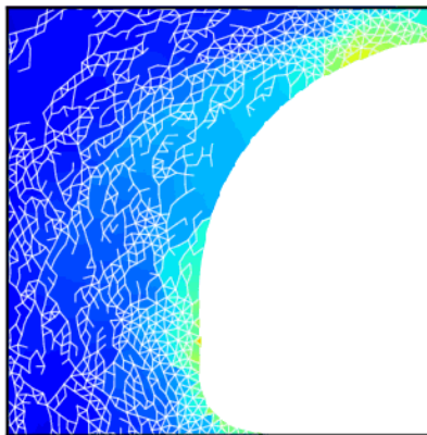
Serrage aux reins (squeezing)
