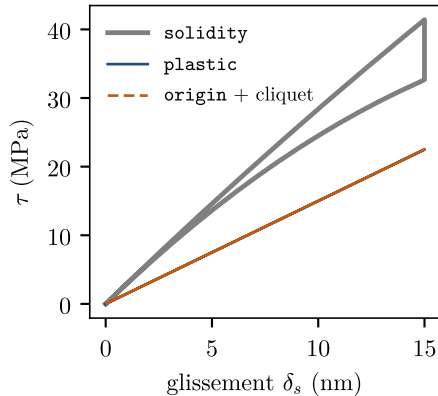
(b) cycle intact, D = 0
