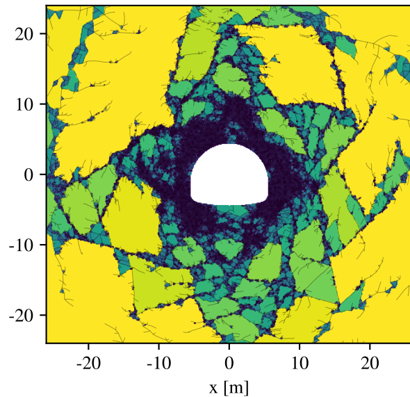
intrinsique (tous joints des t = 0) t = 0.54 s, 35906 joints rompus
