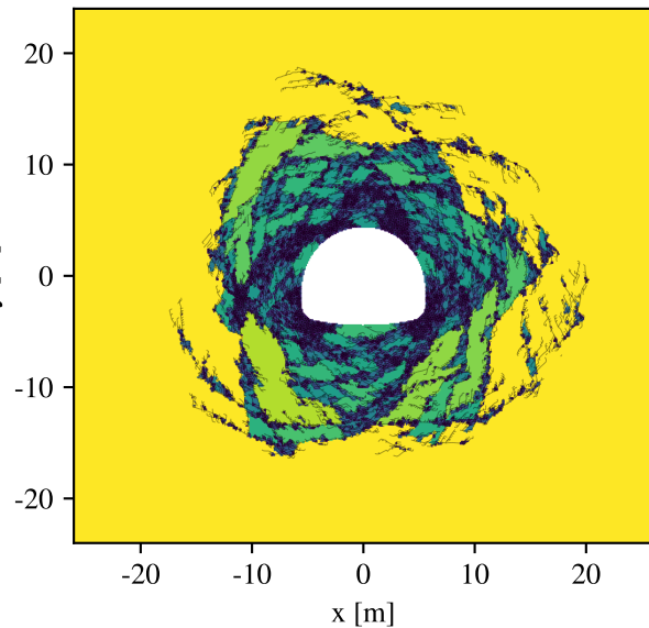
adaptatif (reference) t = 0.42 s, 21378 joints rompus
