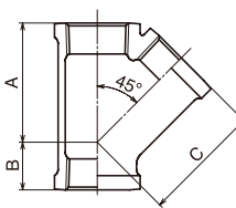
Y Baranches 45° Banded
