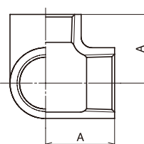
Side Outlet Elbows Banded *
