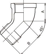
Street Elbows 45° Banded Equal
