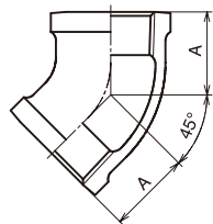
Elbows 45° Banded Equal
