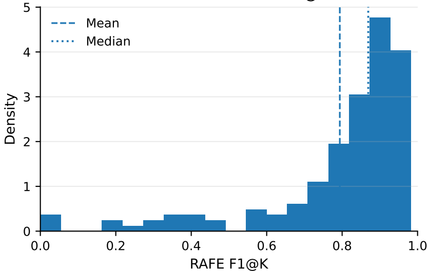
Distribution of RAFE F1@K
