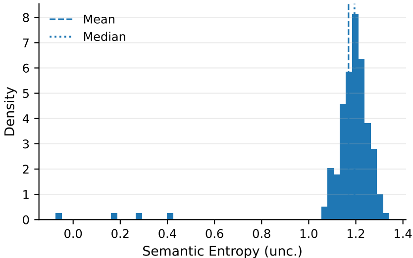
Distribution of Semantic Entropy (unc.)
