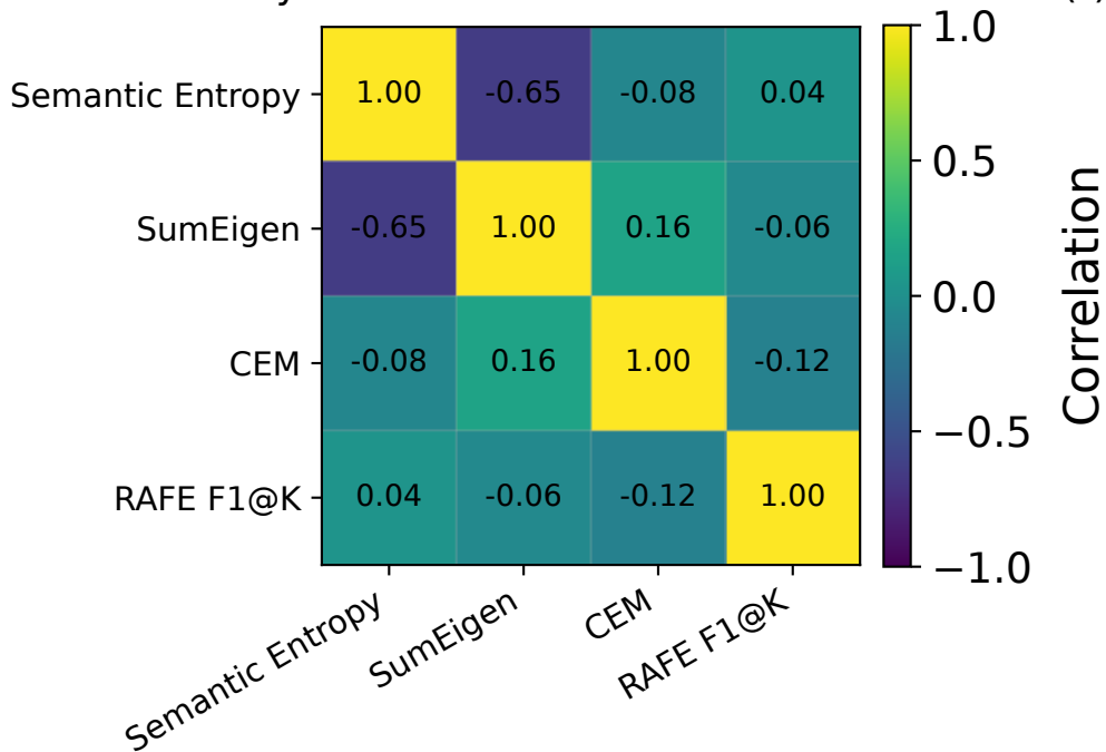
Uncertainty metrics and RAFE: Pearson correlation (r)
