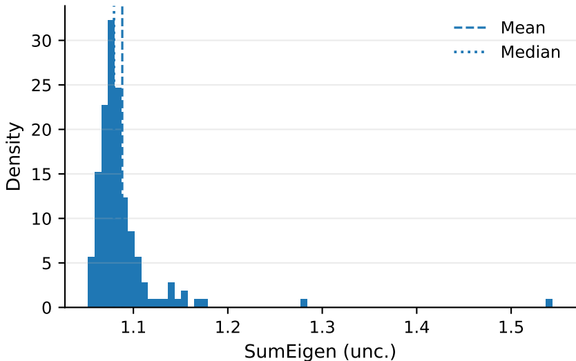
Distribution of SumEigen (unc.)
