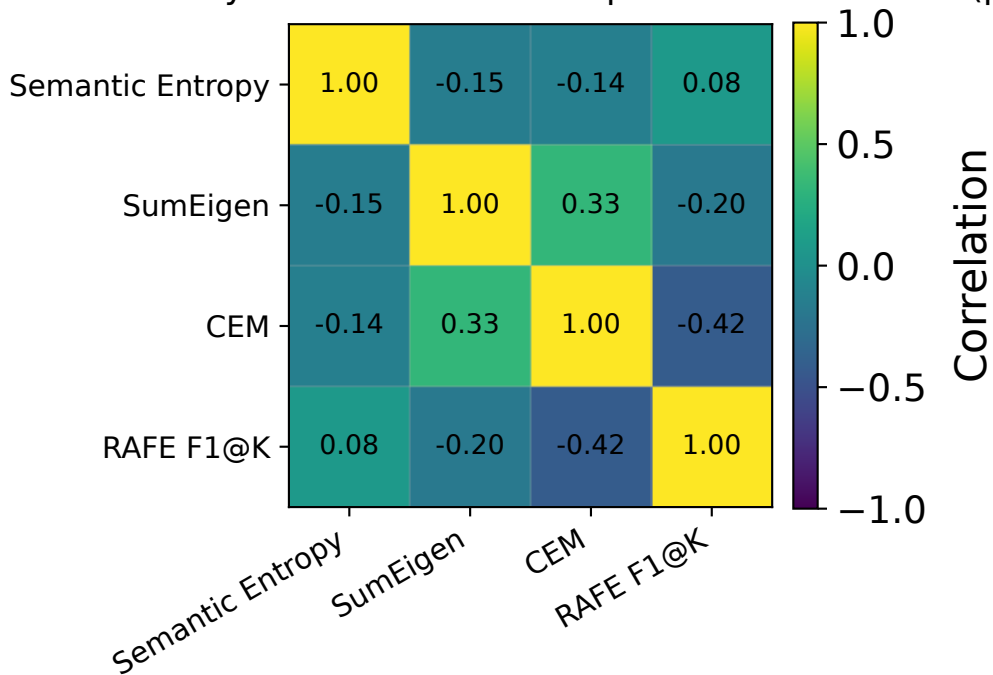
Uncertainty metrics and RAFE: Spearman correlation ( \rho )
