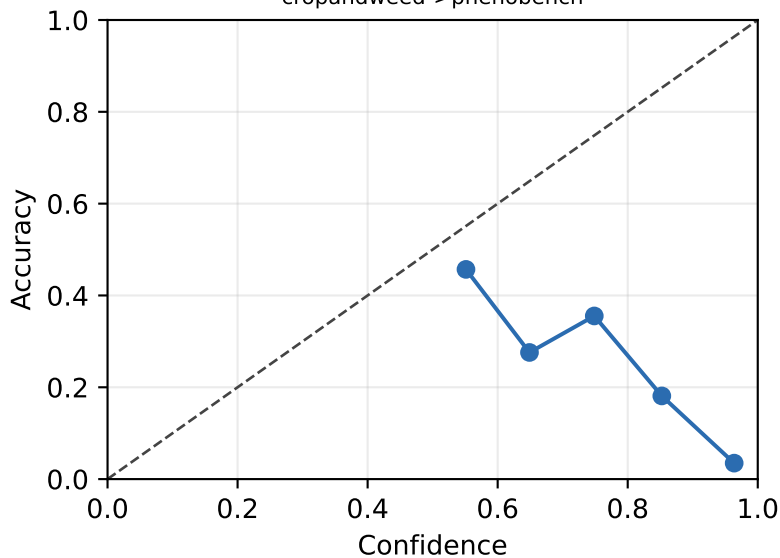
Worst high-confidence transfer Swin-T cropandweed->phenobench
