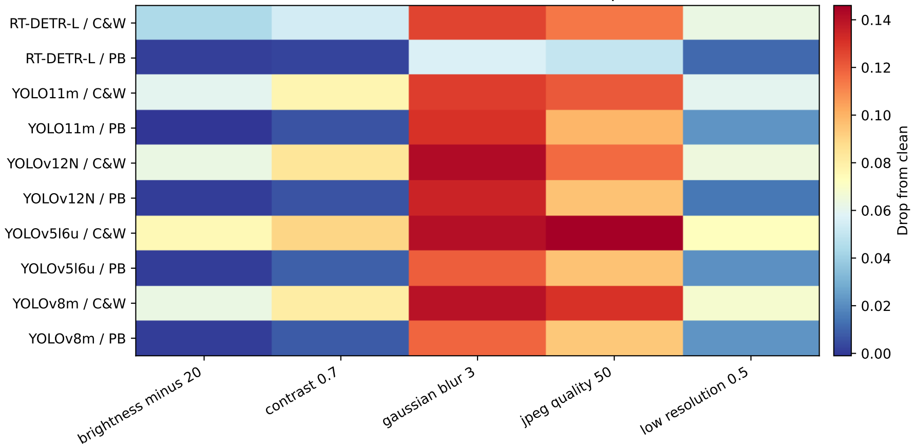
Detection mAP50-95 stress drop
