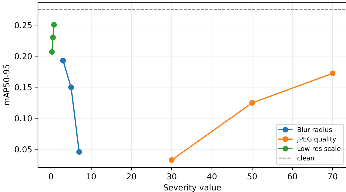
Cross-dataset detection severity audit
