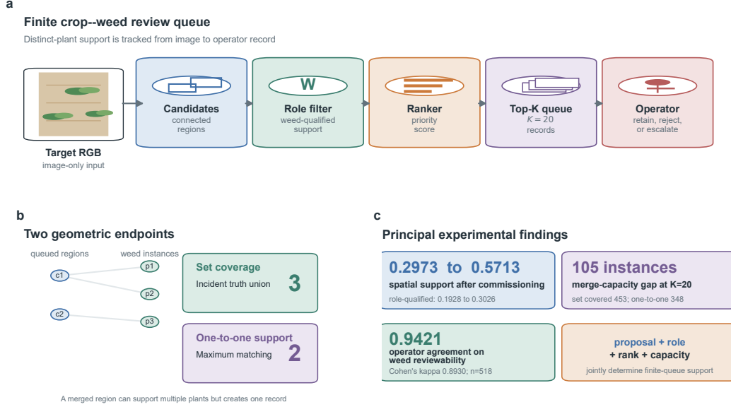
Figure 1: Finite crop–weed review queue and bounded instance-support evaluation. (a) RGB input passes through candidate formation, role qualification, ranking, and a top- K queue before operator review. (b) At fixed K and matching thresholds, set coverage is the incident truth-instance union, whereas one-to-one support is the maximum candidate–instance matching cardinality. (c) Proposal commissioning increased spatial support from 0.2973 to 0.5713; merge-aware matching exposed a 105-instance capacity gap at K = 20 ; and two operators reached 0.9421 agreement on weed reviewability.
