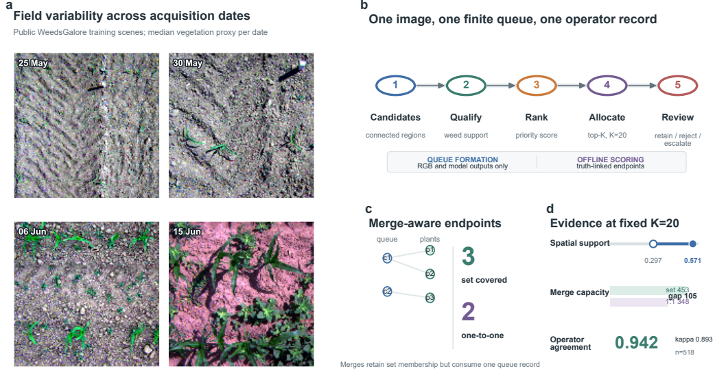
Figure 1: Finite crop–weed review queue and bounded instance-support evaluation. (a) Public WeedsGalore training scenes from four acquisition dates, selected at the within-date median vegetation proxy. (b) Candidate formation, qualification, ranking, and fixed-capacity allocation produce one record per reviewed region; truth enters offline scoring only. (c) Set coverage retains incident truth instances, whereas one-to-one support is the maximum matching cardinality. (d) Commissioning raised spatial support from 0.2973 to 0.5713; merge-aware support was 453 set-covered versus 348 one-to-one instances; operator agreement was 0.9421.
