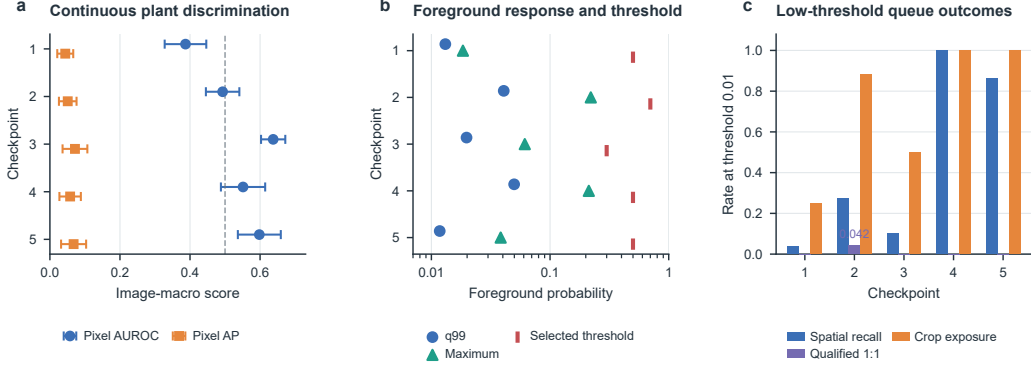
Figure 5: External CWFID transfer across five U-Net checkpoints. (a) Image-macro plant-pixel AUROC and AP; error bars show the sample SD across 60 images. (b) Image-macro foreground q_{0.99} and maximum probabilities relative to the validation-selected threshold. (c) Spatial recall, role-qualified one-to-one recall, and crop-exposure image frequency at threshold 0.01. Checkpoints follow the predefined evaluation order.
