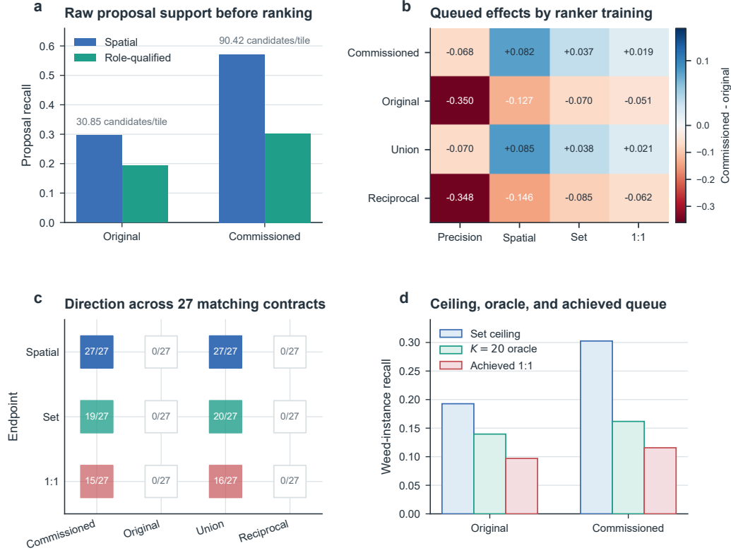
Figure 2: Proposal and ranker sensitivity. (a) Raw spatial and role-qualified proposal support before ranking. (b) Commissioned-minus-original effects under four ranker-training schemes. (c) Cells report the number of positive effects among 27 matching contracts. (d) Ranker-free set ceiling, per-tile K = 20 oracle, and achieved one-to-one support for the commissioned-only ranker.
