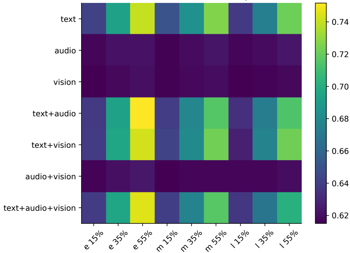
MAE (common feasible samples)
