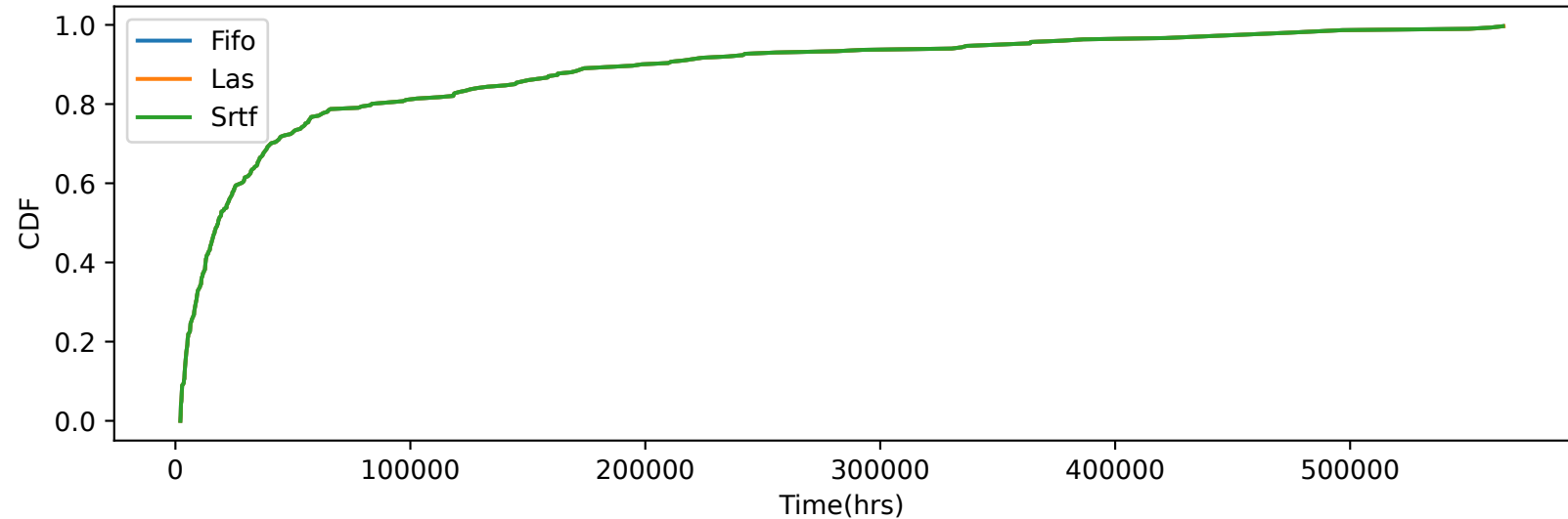
Srtf_load_5.0_cdf
