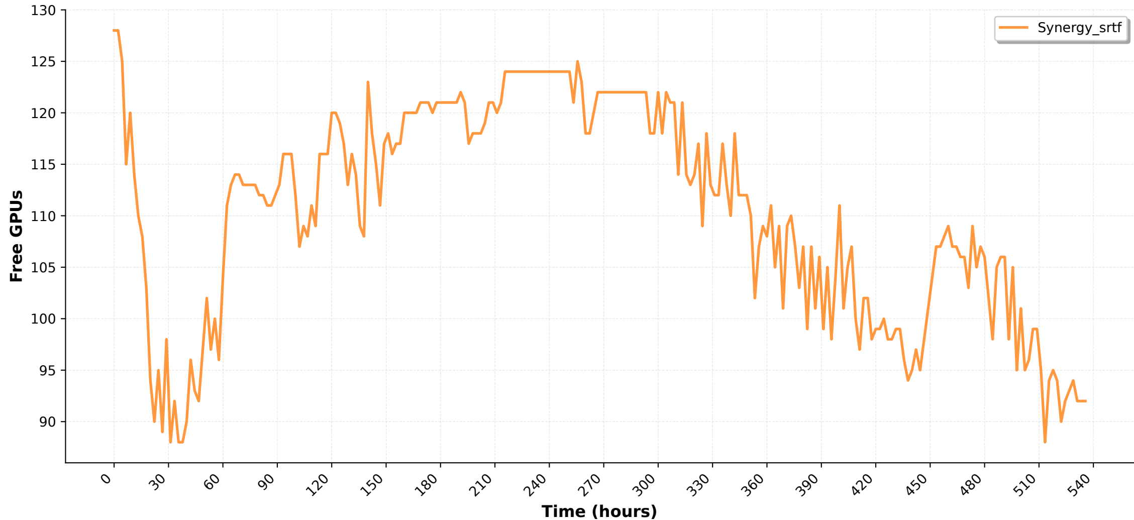
Free GPUs Over Time (Load: 5.0 jobs/hour, Scheduler: Synergy_srtf)
