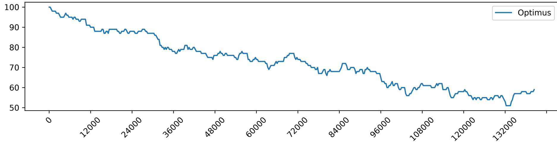
Optimus_load_4.0_free_GPUs
