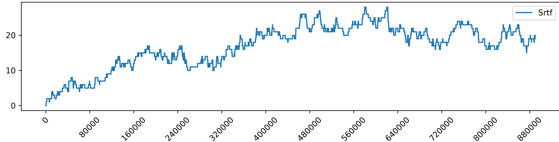
Srtf_load_1.0_gpu_demand
