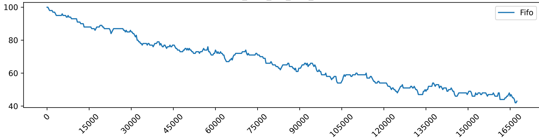
Fifo_load_4.0_free_GPUs
