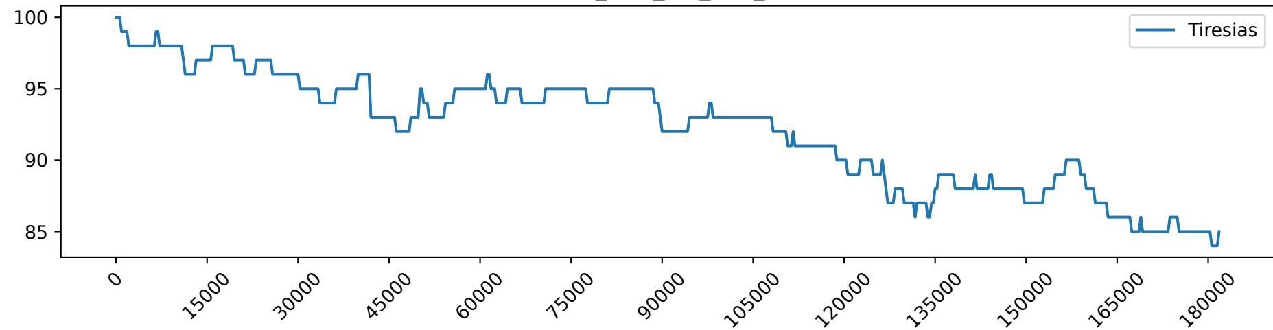
Tiresias_load_1.0_free_GPUs
