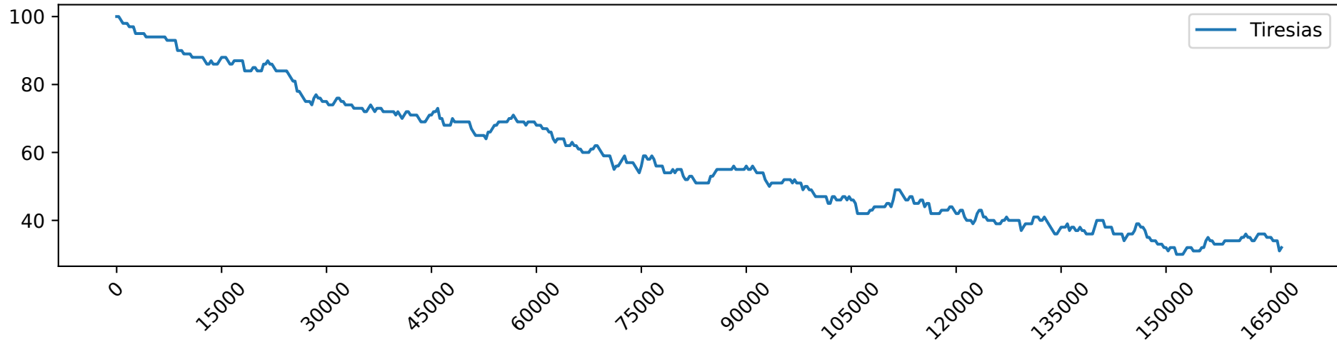
Tiresias_load_5.0_free_GPUs
