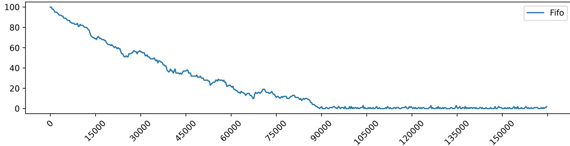
Fifo_load_10.0_free_GPUs
