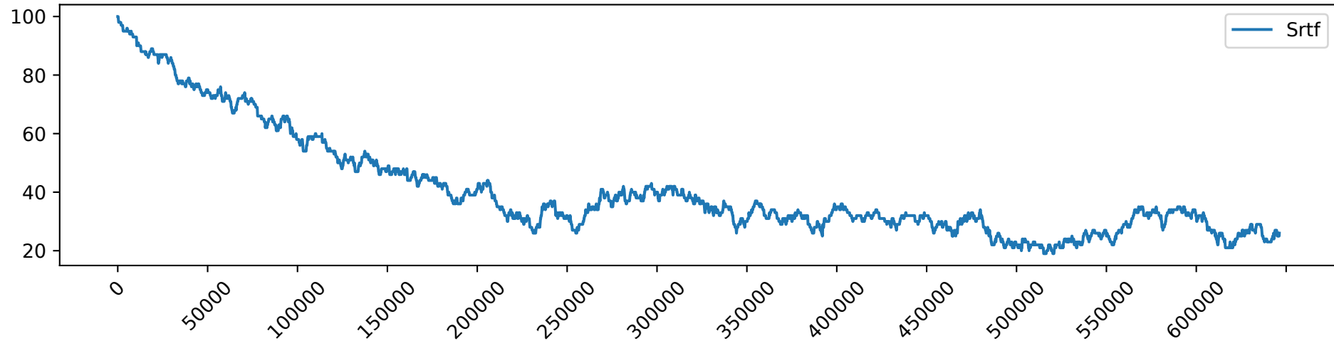
Srtf_load_4.0_free_GPUs
