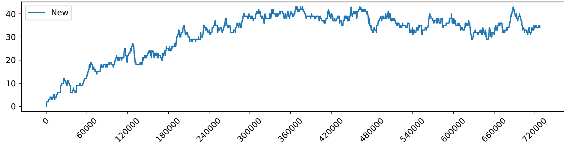
New_load_2.0_gpu_demand
