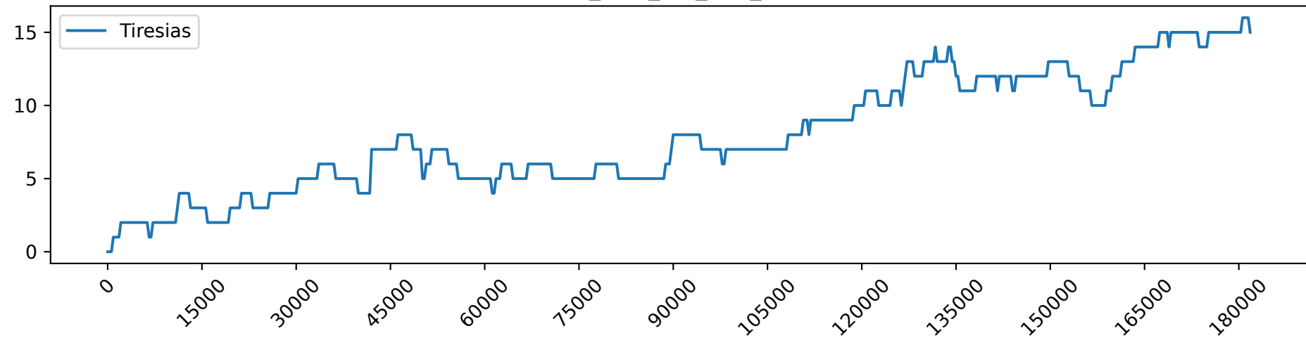
Tiresias_load_1.0_gpu_demand
