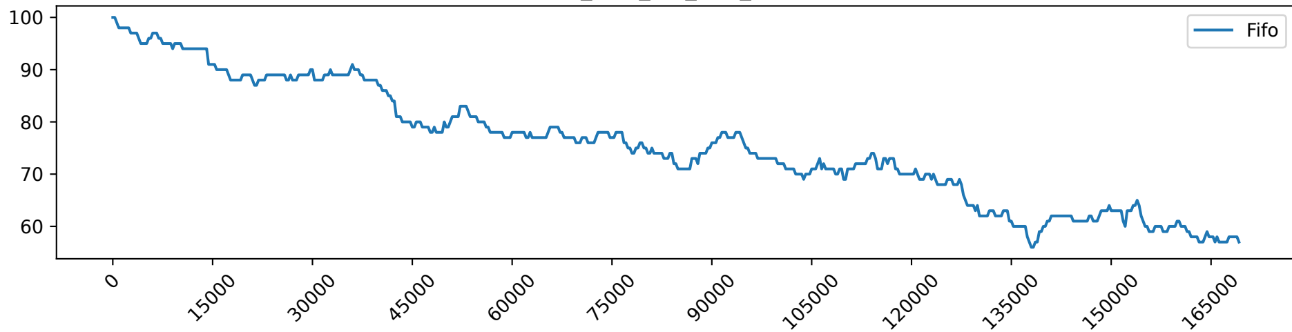
Fifo_load_3.0_free_GPUs
