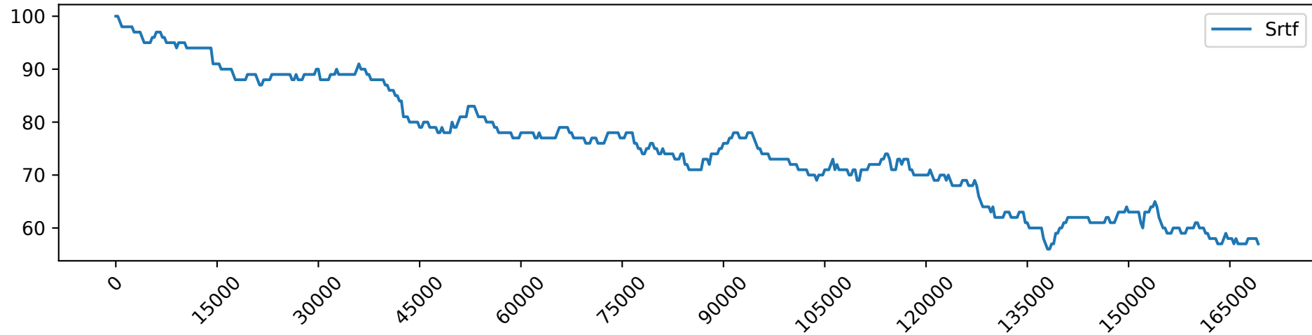
Srtf_load_3.0_free_GPUs
