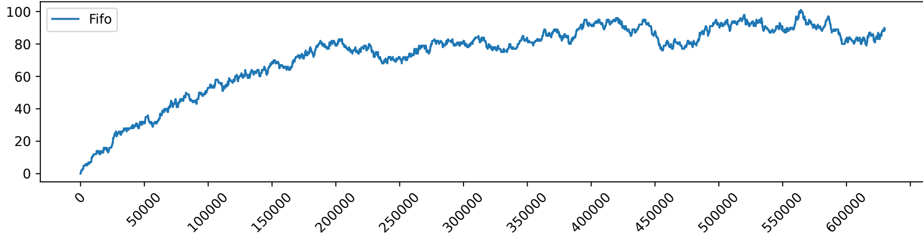
Fifo_load_5.0_gpu_demand
