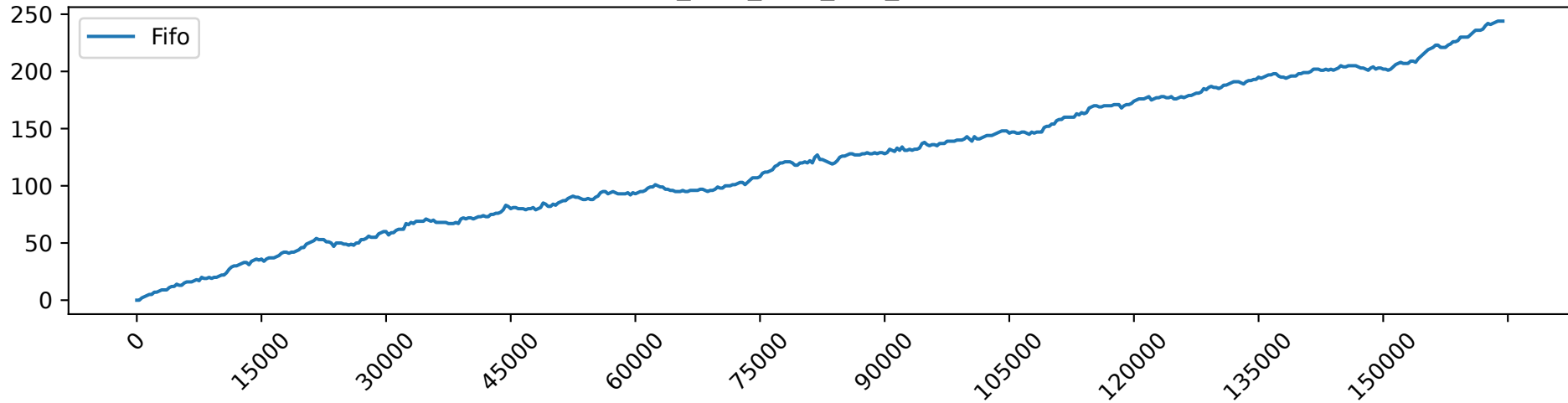
Fifo_load_12.0_gpu_demand
