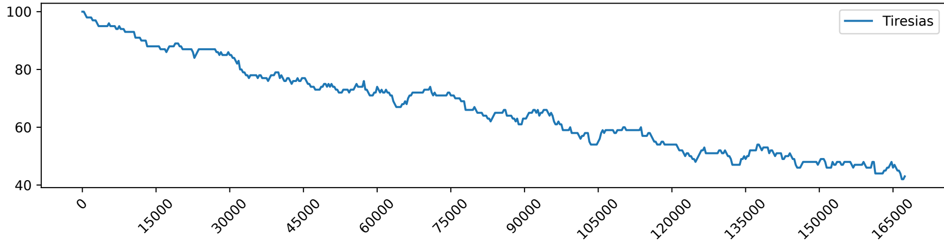
Tiresias_load_4.0_free_GPUs
