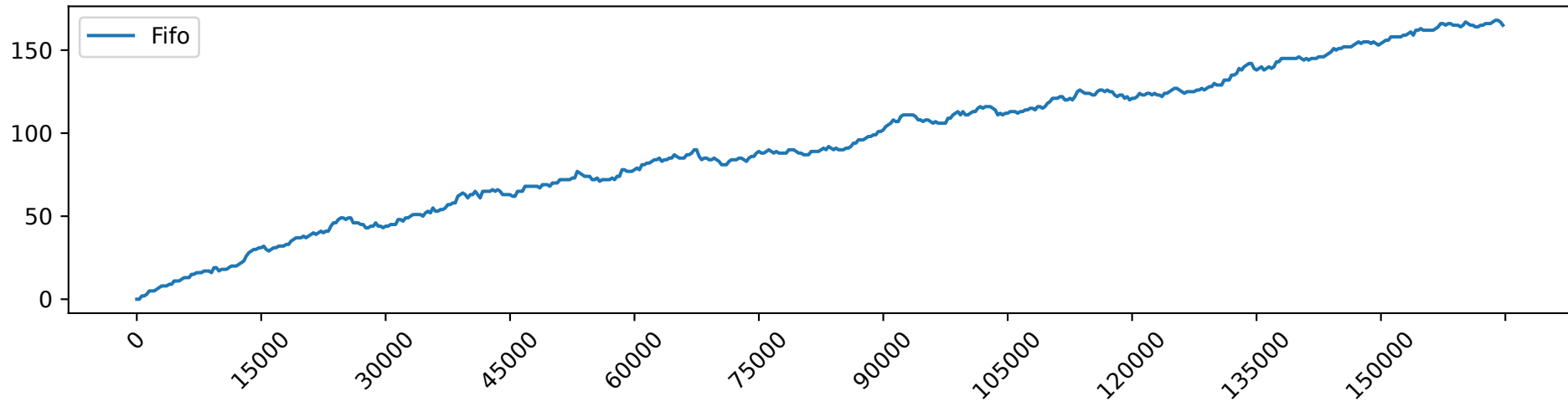
Fifo_load_10.0_gpu_demand
