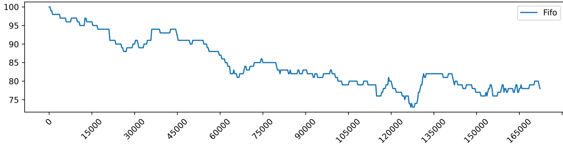
Fifo_load_2.0_free_GPUs
