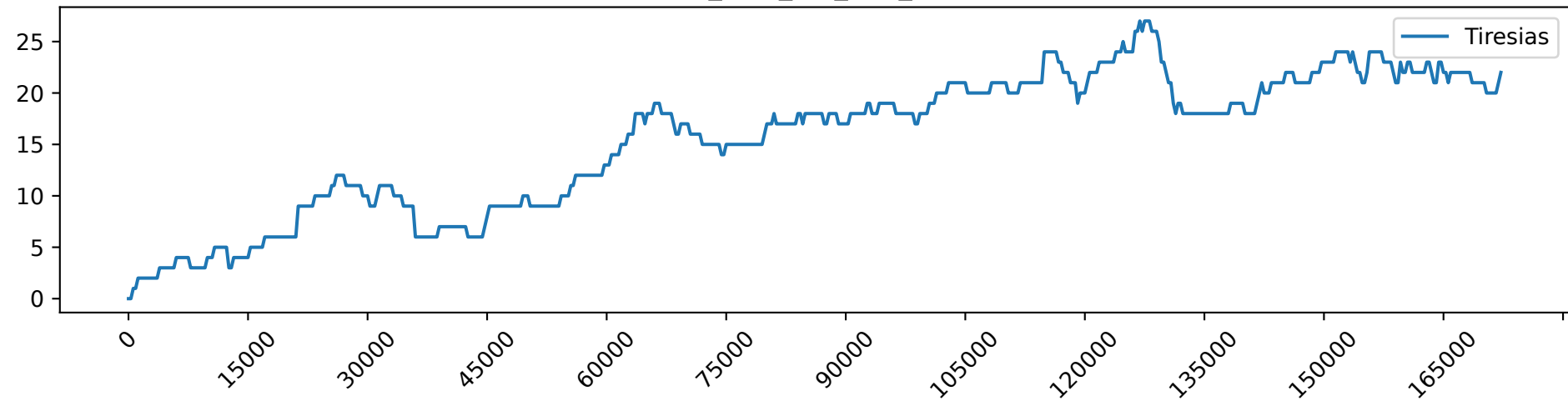
Tiresias_load_2.0_gpu_demand
