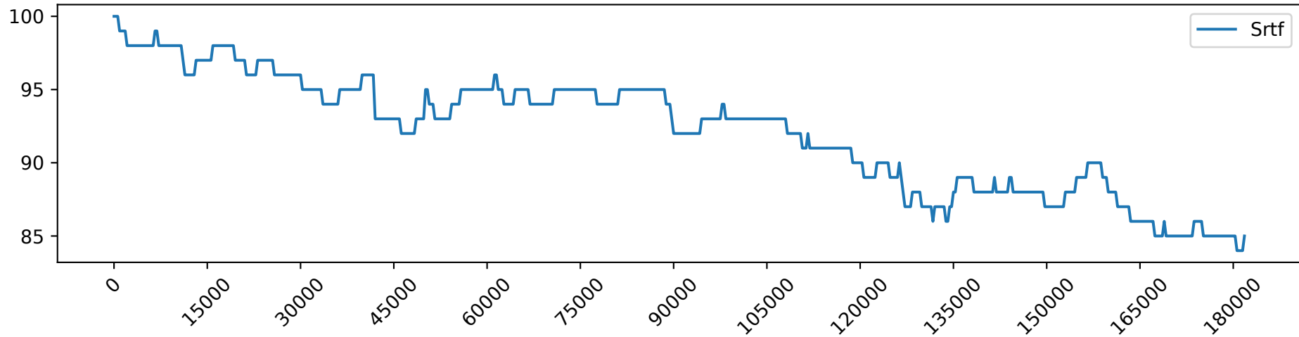
Srtf_load_1.0_free_GPUs
