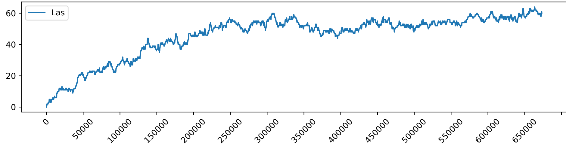
Las_load_3.0_gpu_demand
