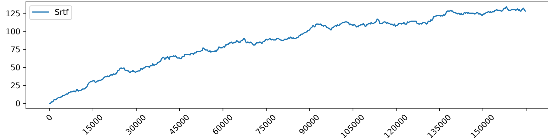
Srtf_load_10.0_gpu_demand
