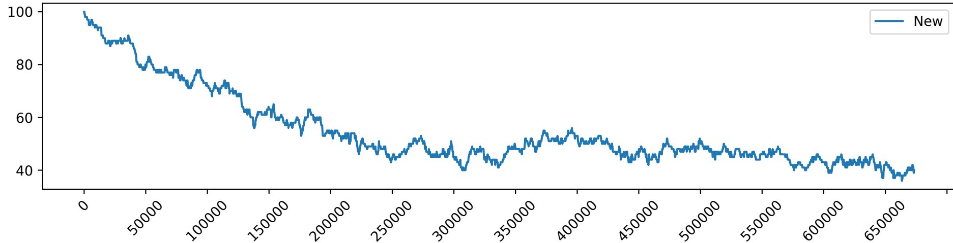
New_load_3.0_free_GPUs
