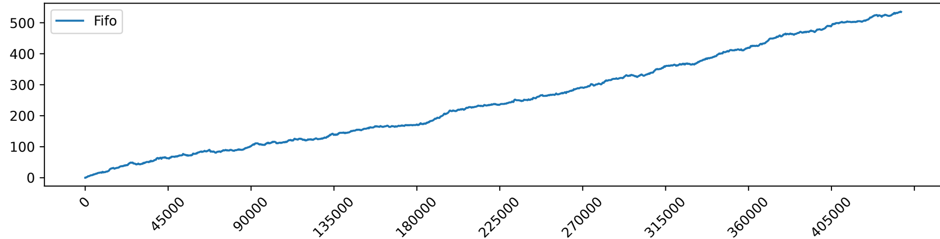
Fifo_load_10.0_gpu_demand
