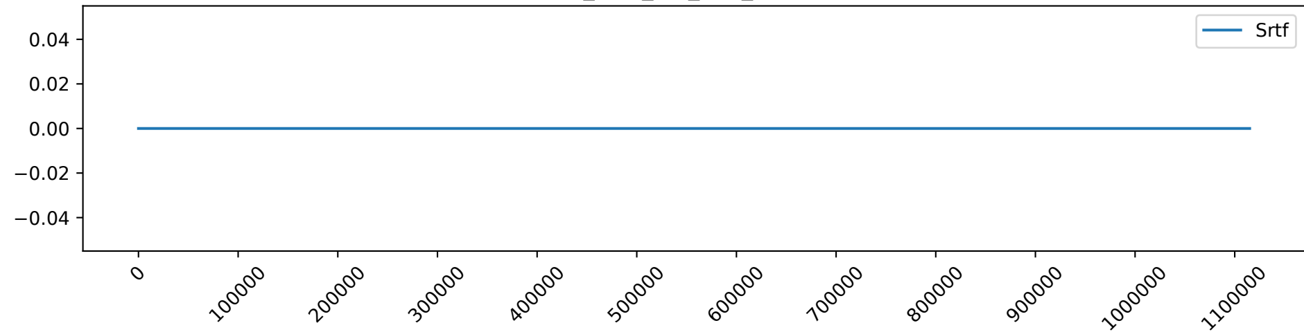
Srtf_load_5.0_gpu_demand
