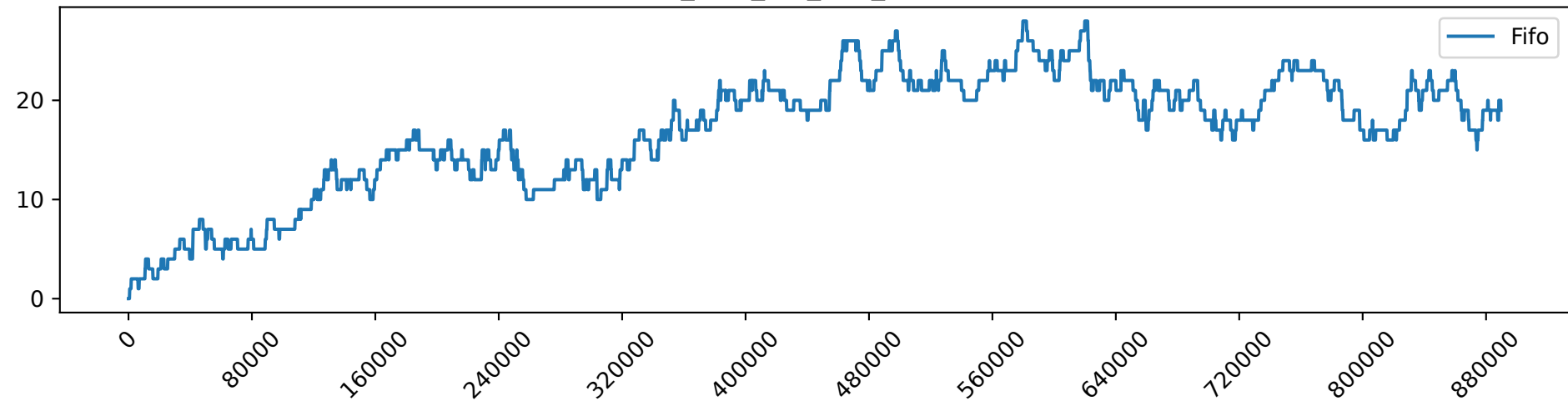
Fifo_load_1.0_gpu_demand
