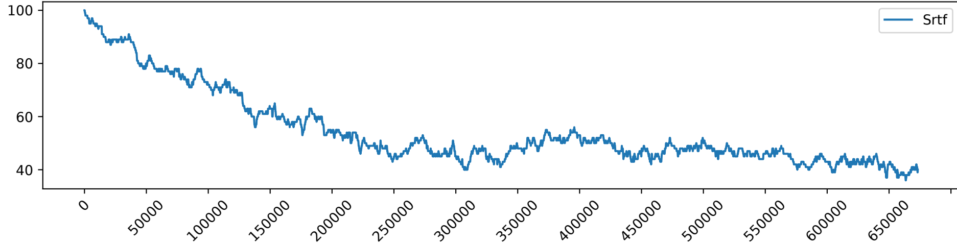
Srtf_load_3.0_free_GPUs
