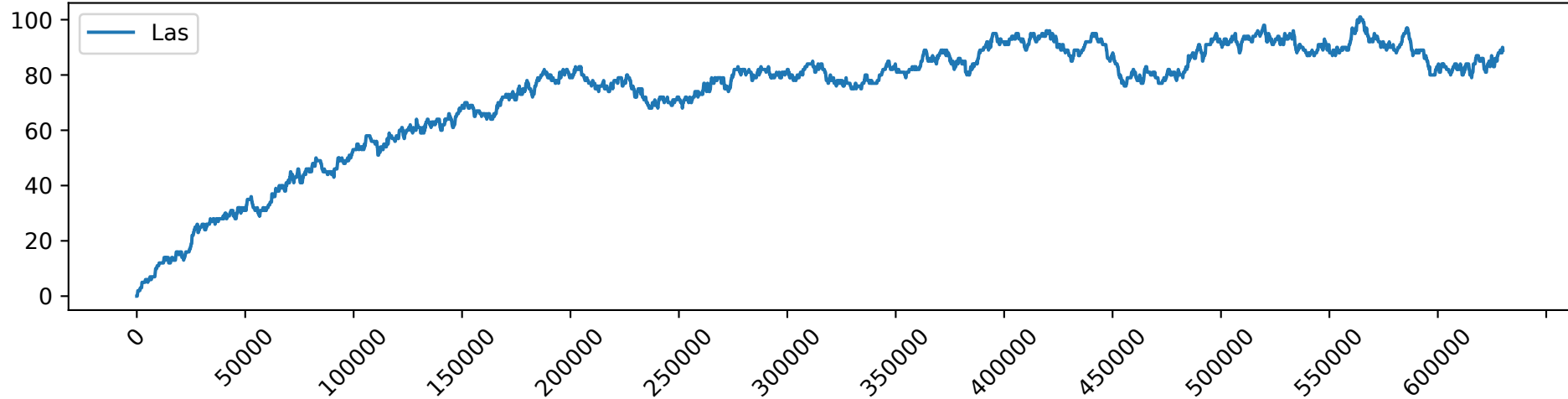
Las_load_5.0_gpu_demand
