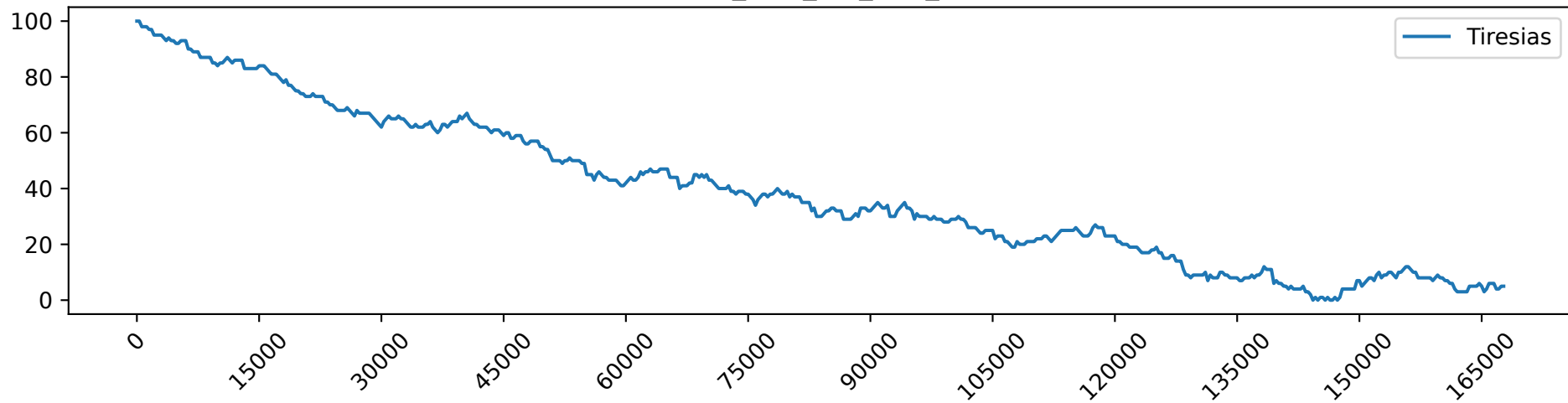
Tiresias_load_7.0_free_GPUs
