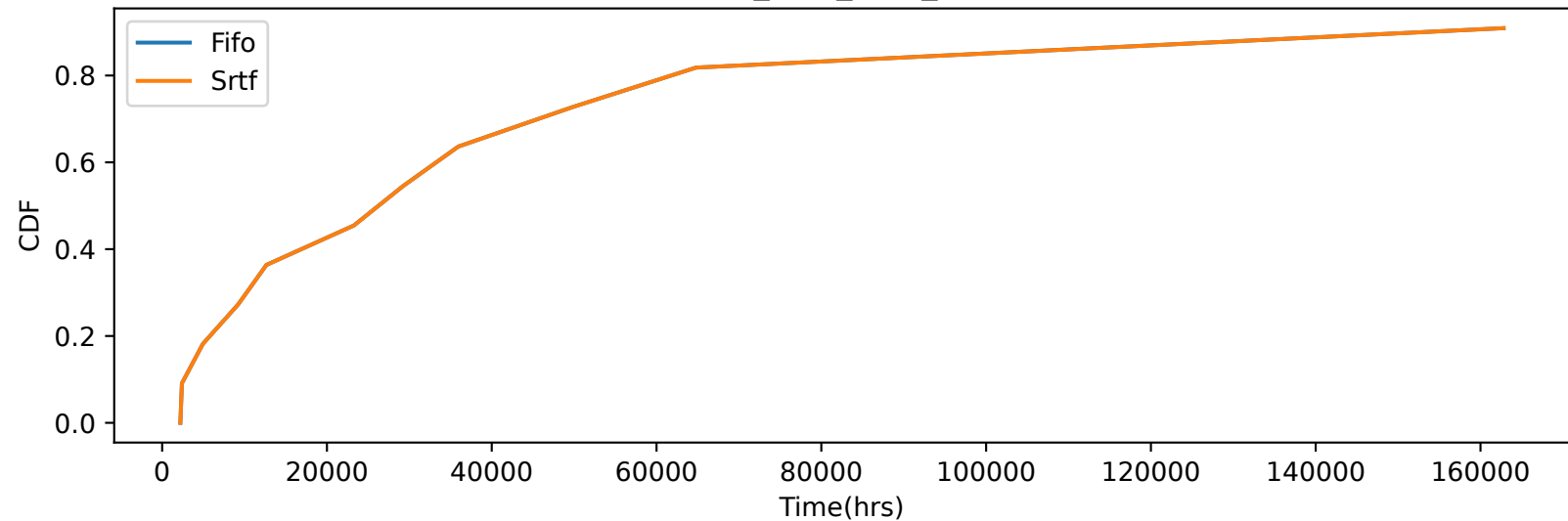
Srtf_load_10.0_cdf
