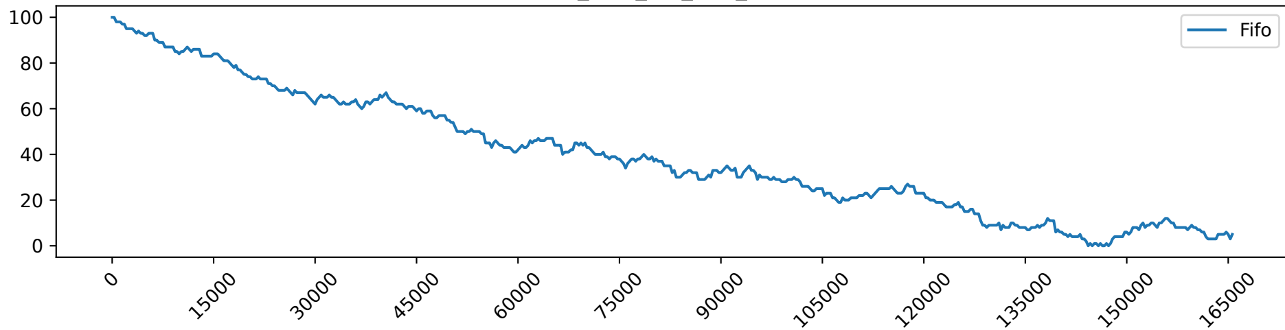
Fifo_load_7.0_free_GPUs
