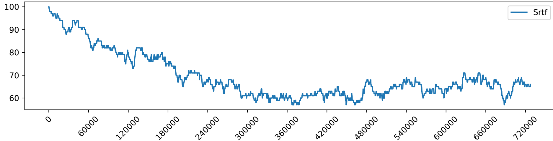
Srtf_load_2.0_free_GPUs
