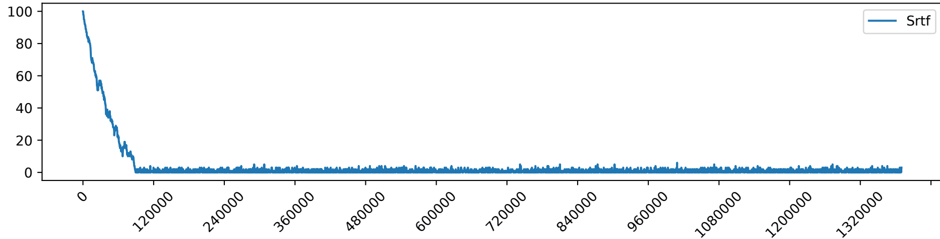
Srtf_load_10.0_free_GPUs
