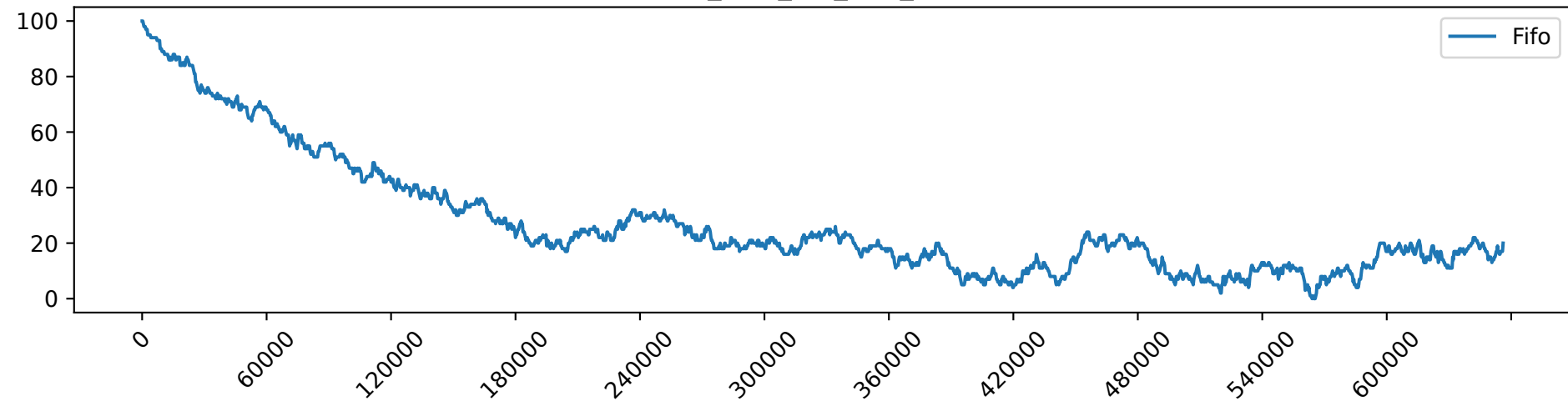
Fifo_load_5.0_free_GPUs
