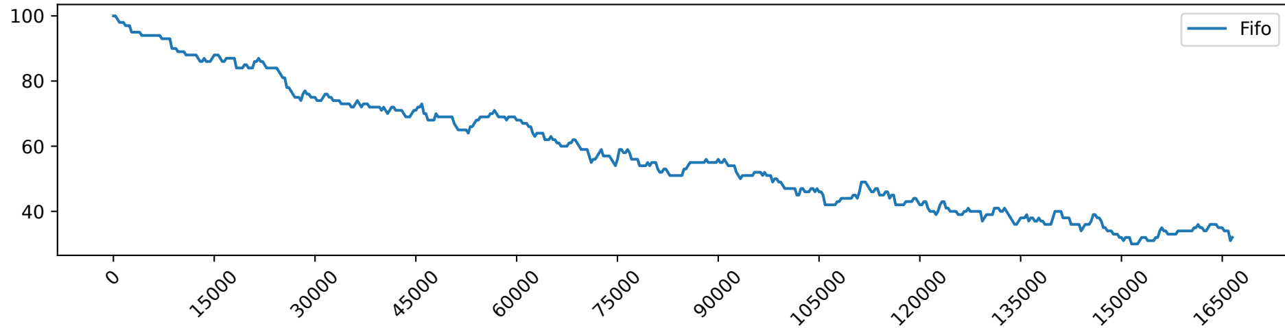
Fifo_load_5.0_free_GPUs
