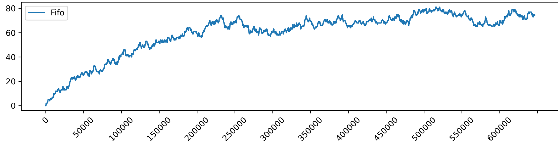
Fifo_load_4.0_gpu_demand
