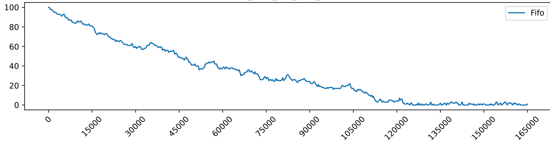
Fifo_load_8.0_free_GPUs
