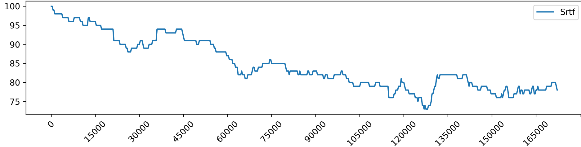
Srtf_load_2.0_free_GPUs
