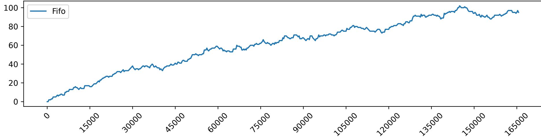
Fifo_load_7.0_gpu_demand
