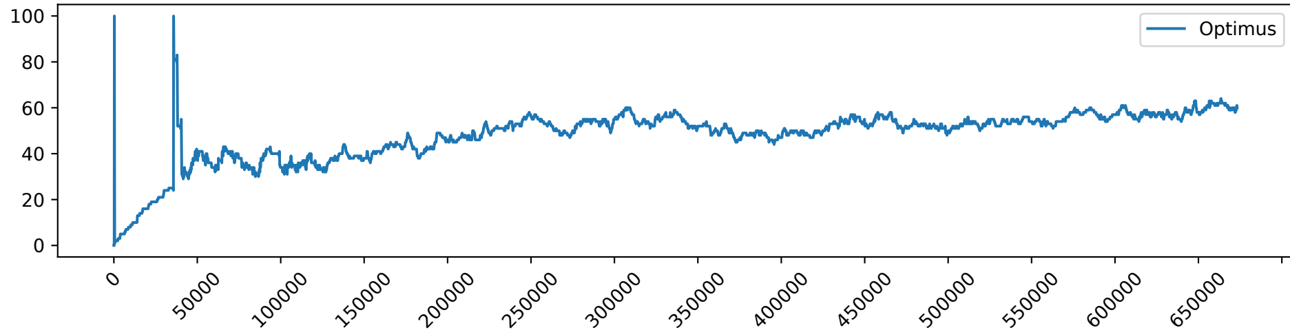
Optimus_load_3.0_gpu_demand
