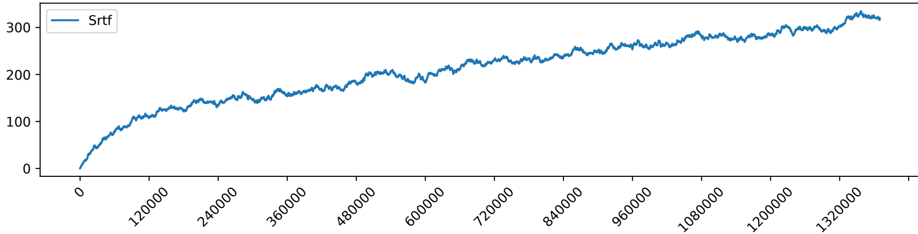
Srtf_load_10.0_gpu_demand
