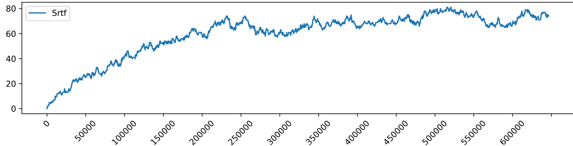
Srtf_load_4.0_gpu_demand
