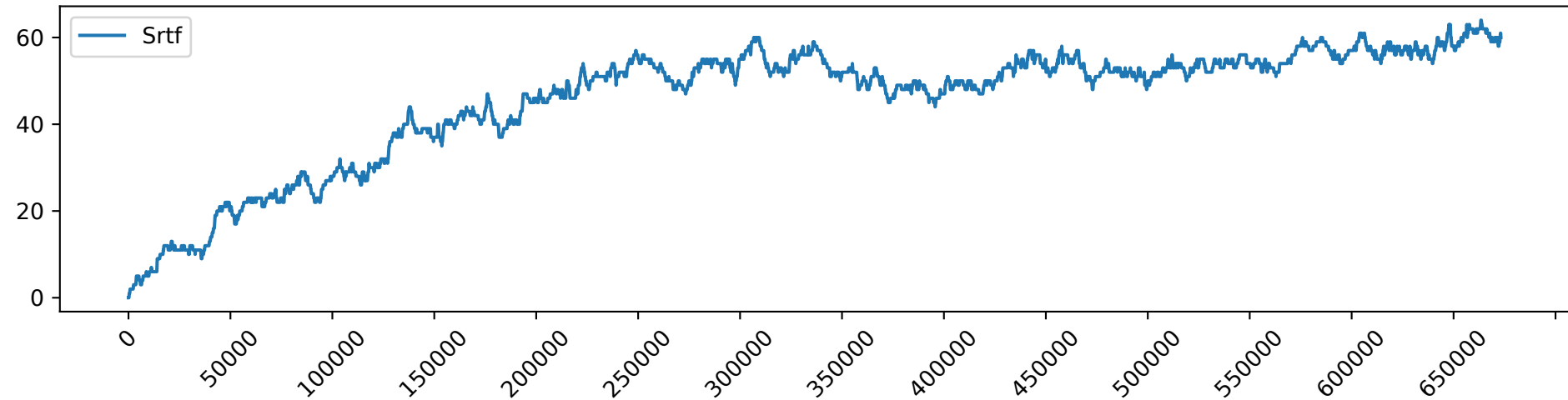
Srtf_load_3.0_gpu_demand
