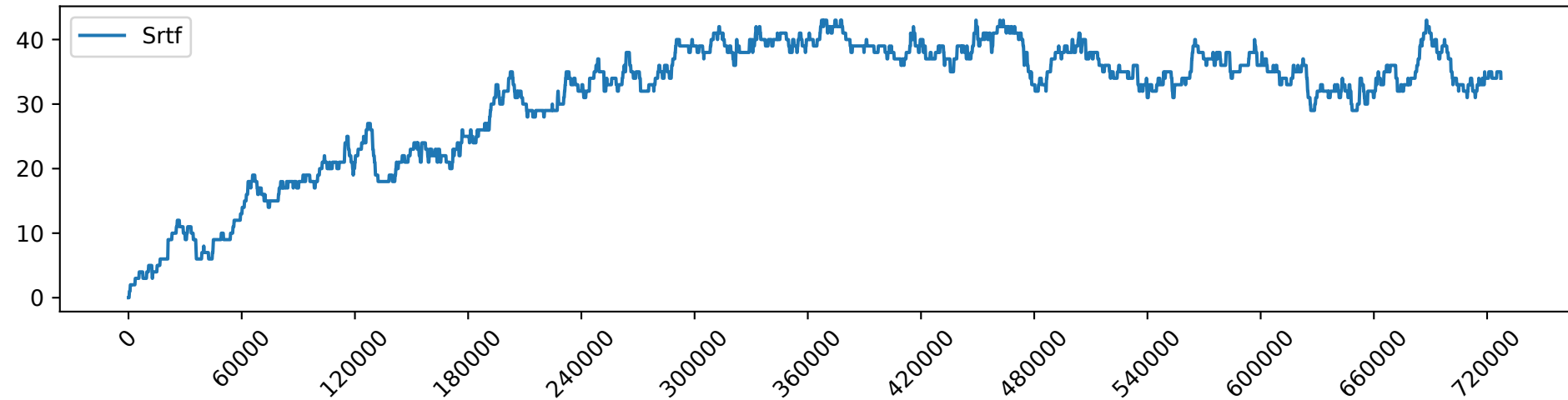
Srtf_load_2.0_gpu_demand
