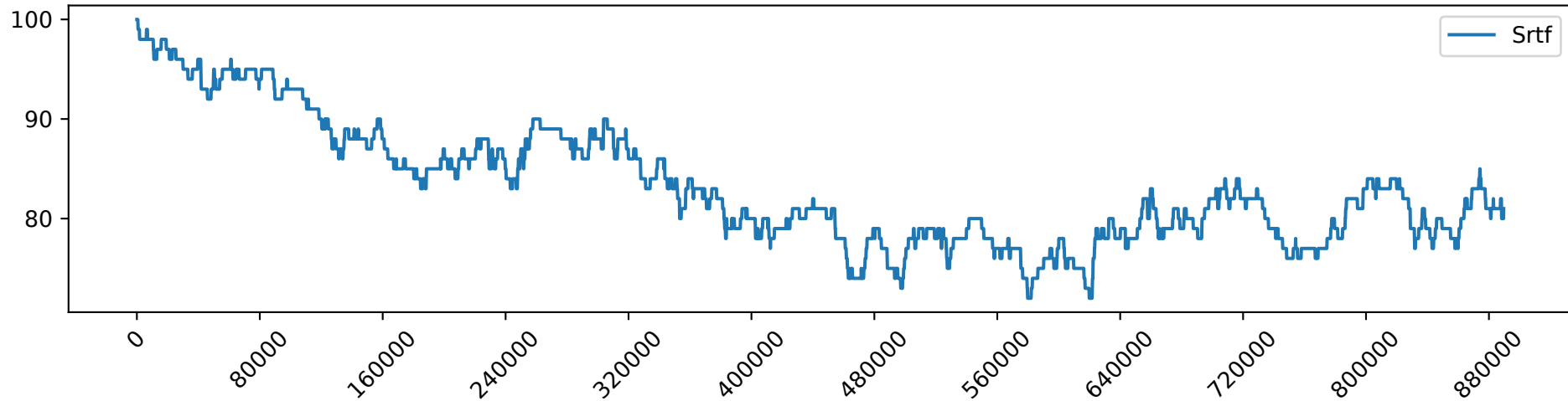
Srtf_load_1.0_free_GPUs
