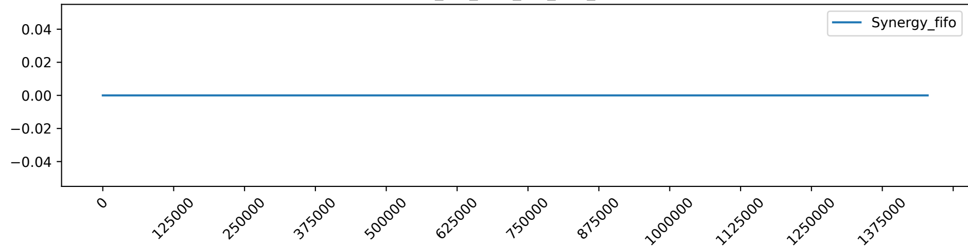
Synergy_fifo_load_9.0_gpu_demand
