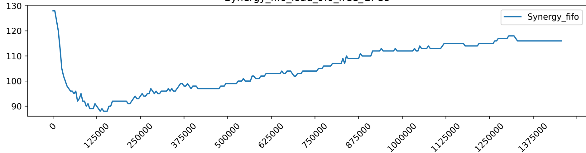
Synergy_fifo_load_9.0_free_GPUs
