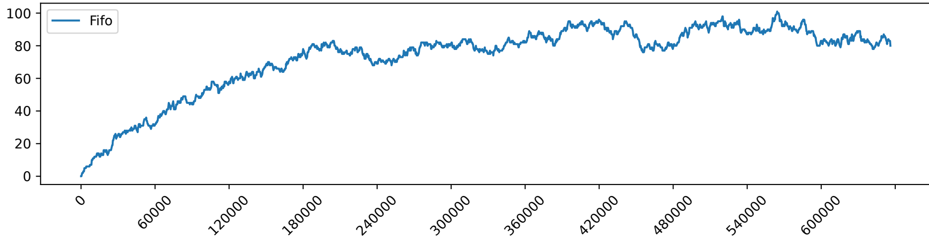
Fifo_load_5.0_gpu_demand
