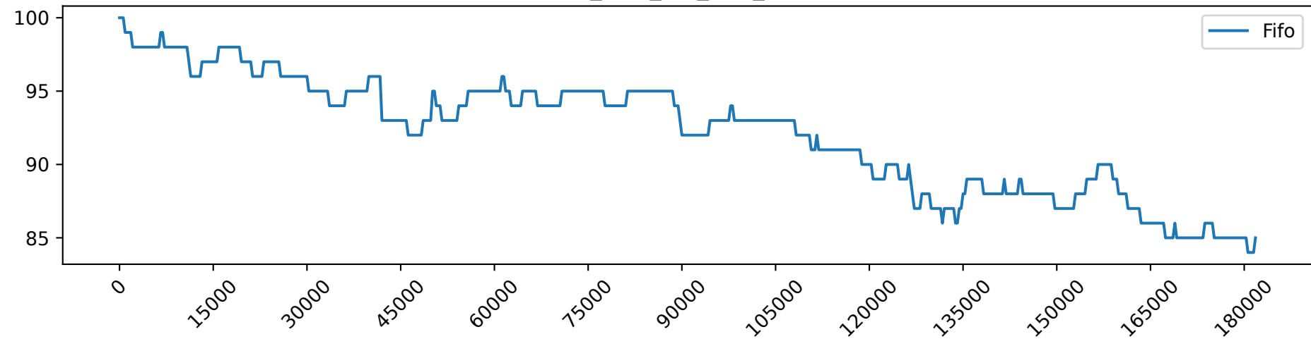
Fifo_load_1.0_free_GPUs
