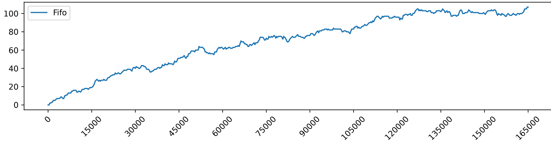
Fifo_load_8.0_gpu_demand
