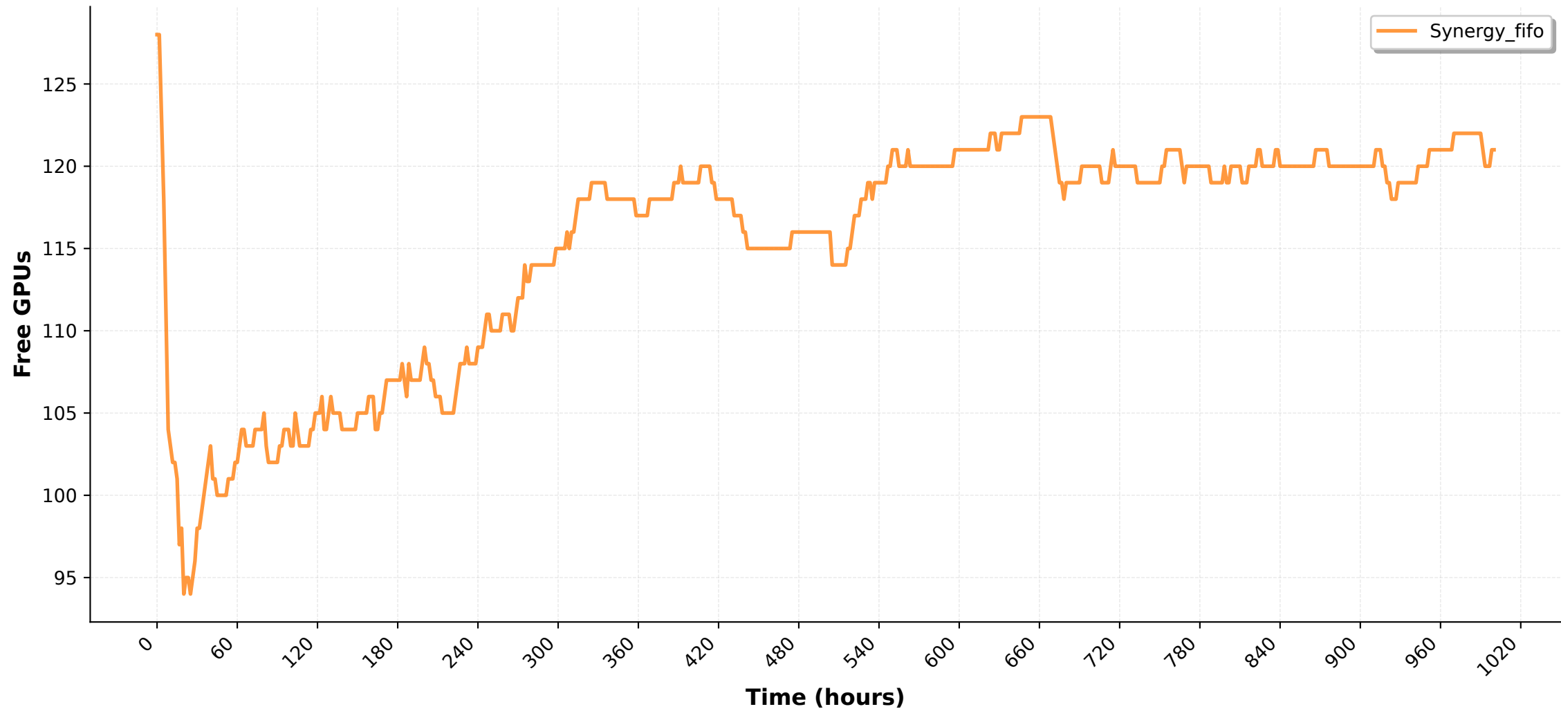
Free GPUs Over Time (Load: 9.0 jobs/hour, Scheduler: Synergy_fifo)
