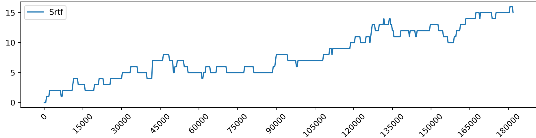
Srtf_load_1.0_gpu_demand
