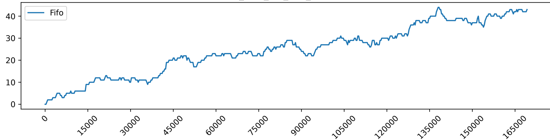
Fifo_load_3.0_gpu_demand
