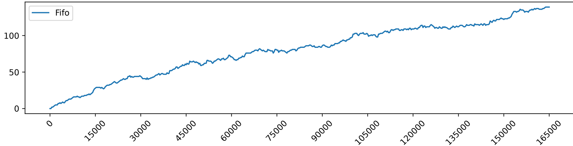
Fifo_load_9.0_gpu_demand
