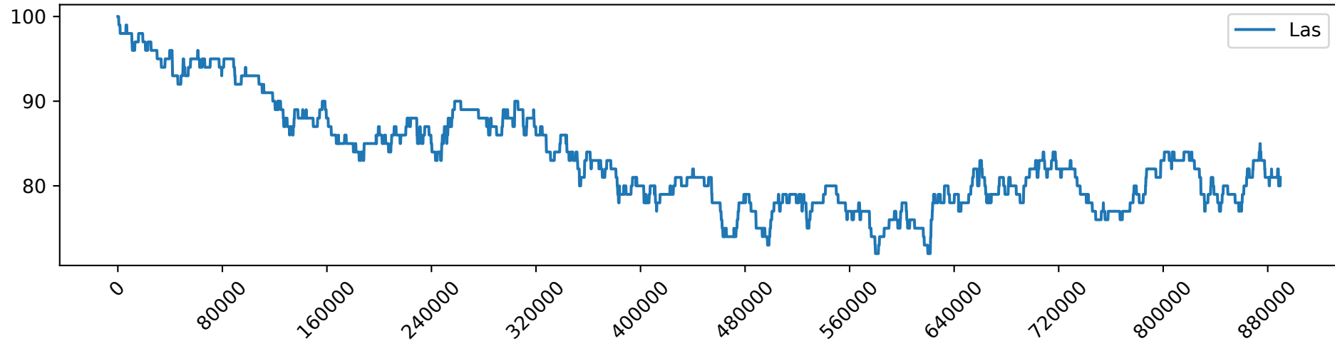
Las_load_1.0_free_GPUs
