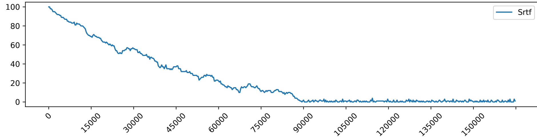
Srtf_load_10.0_free_GPUs
