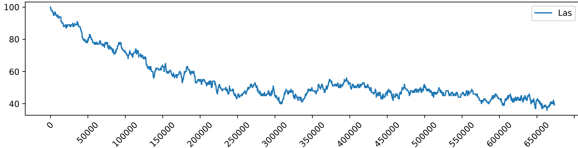
Las_load_3.0_free_GPUs
