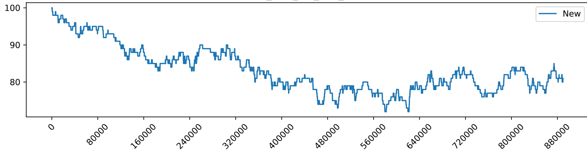
New_load_1.0_free_GPUs
