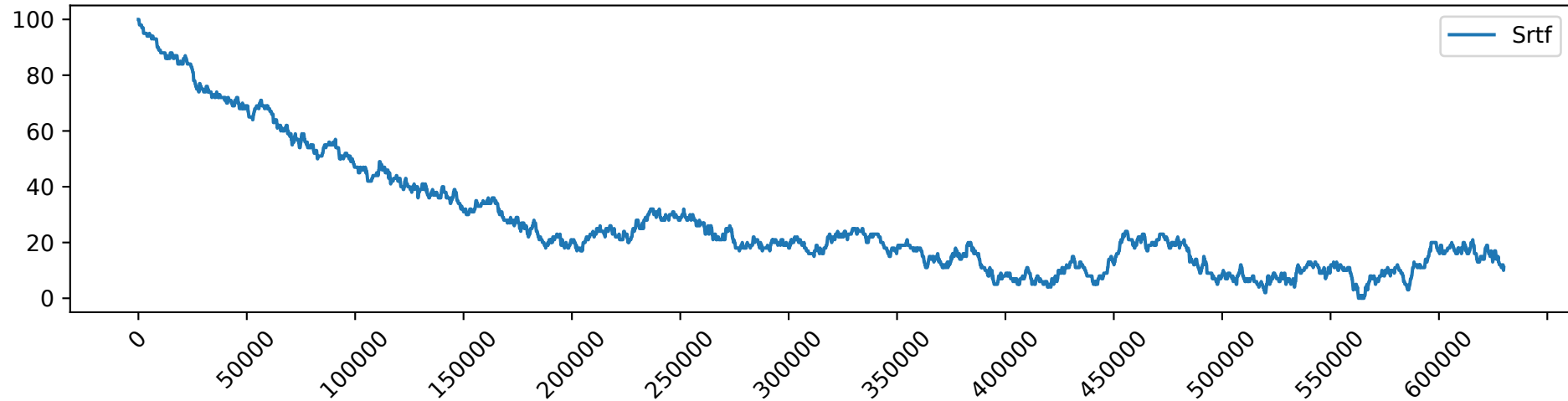
Srtf_load_5.0_free_GPUs
