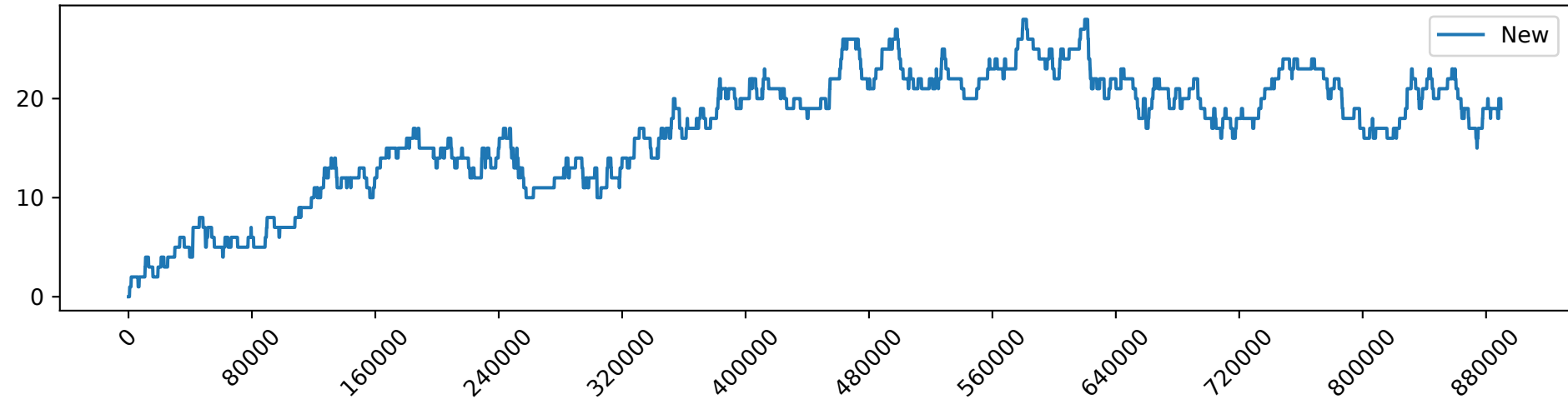
New_load_1.0_gpu_demand
