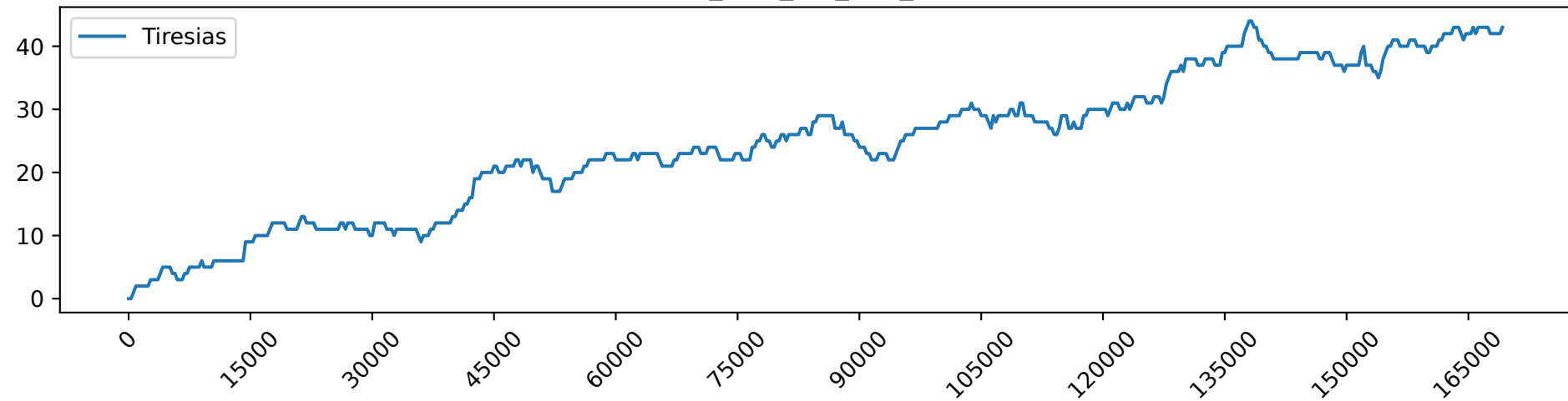
Tiresias_load_3.0_gpu_demand
