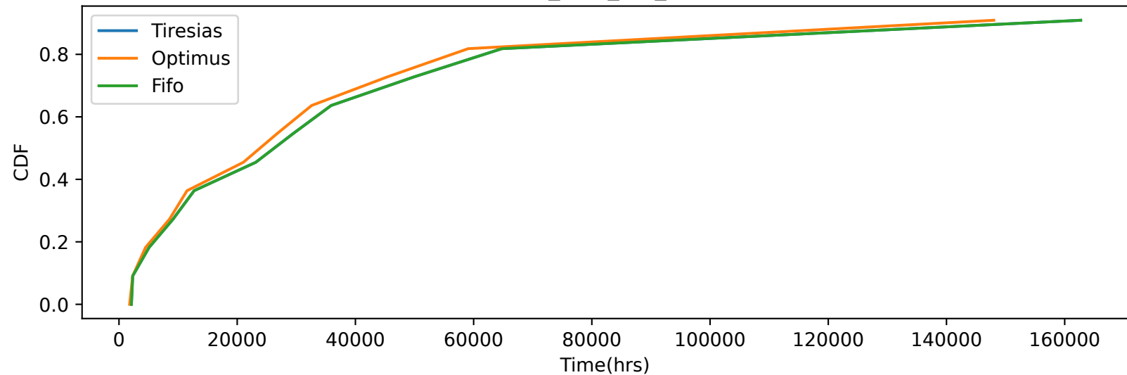
Fifo_load_5.0_cdf
