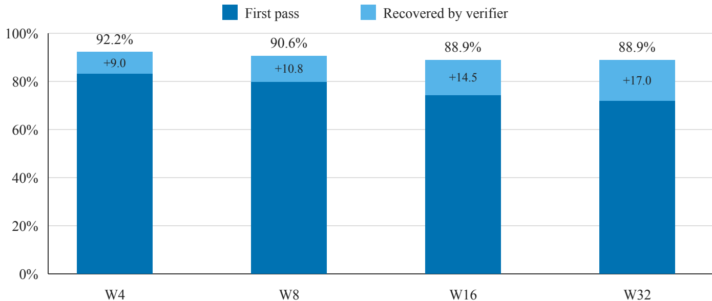
Source coverage
