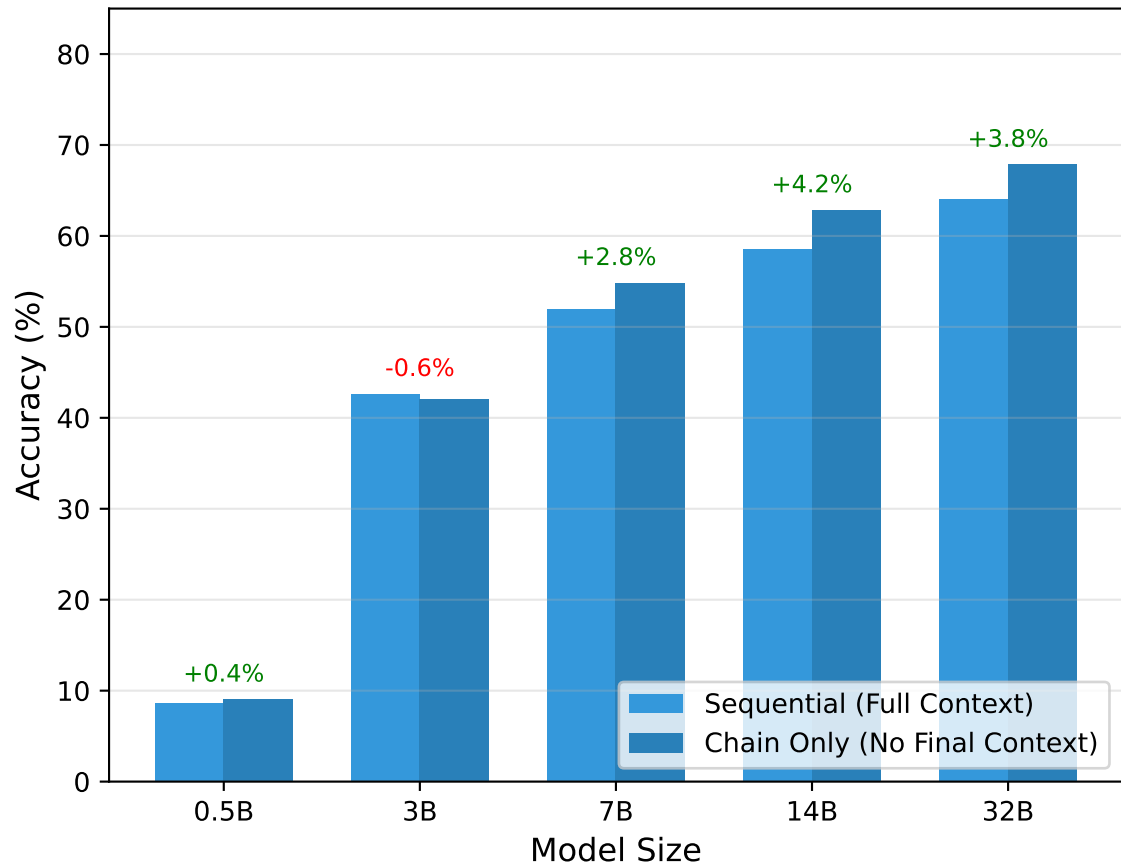
Sequential: Q&amp;A History Sufficiency
