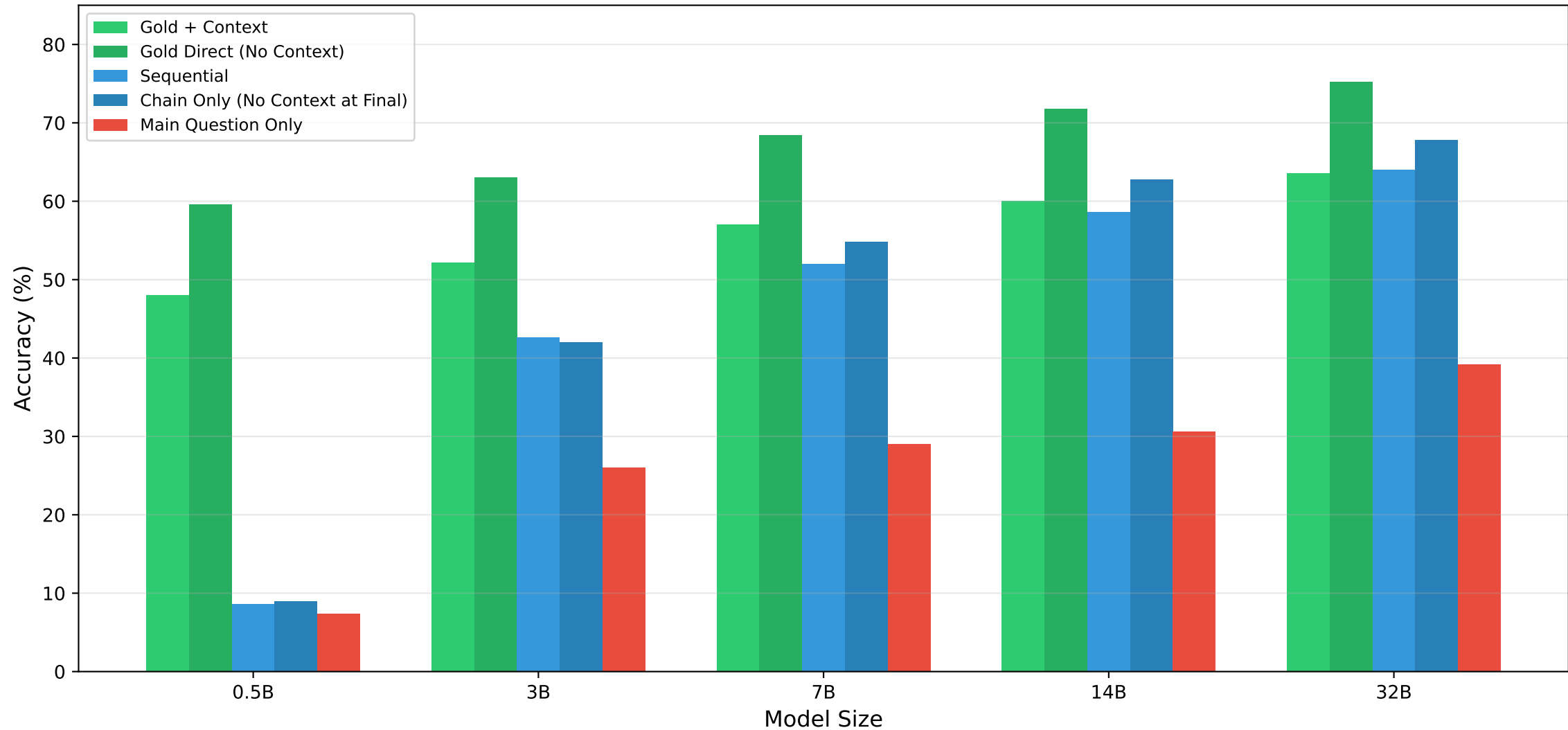
Exp 1: Answer Dependency Study on MoreHopQA
