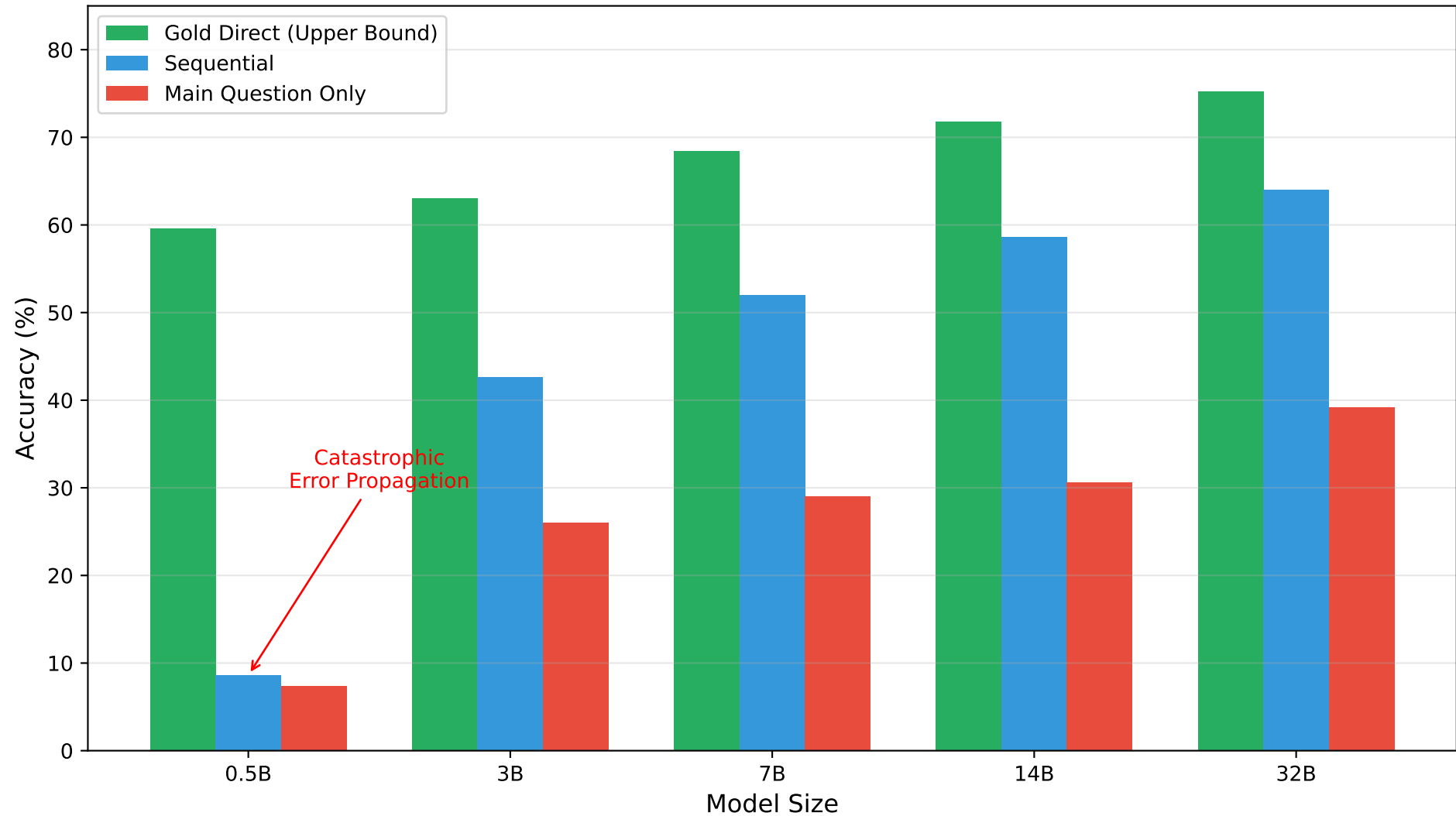
Error Propagation: Small Models Suffer Most
