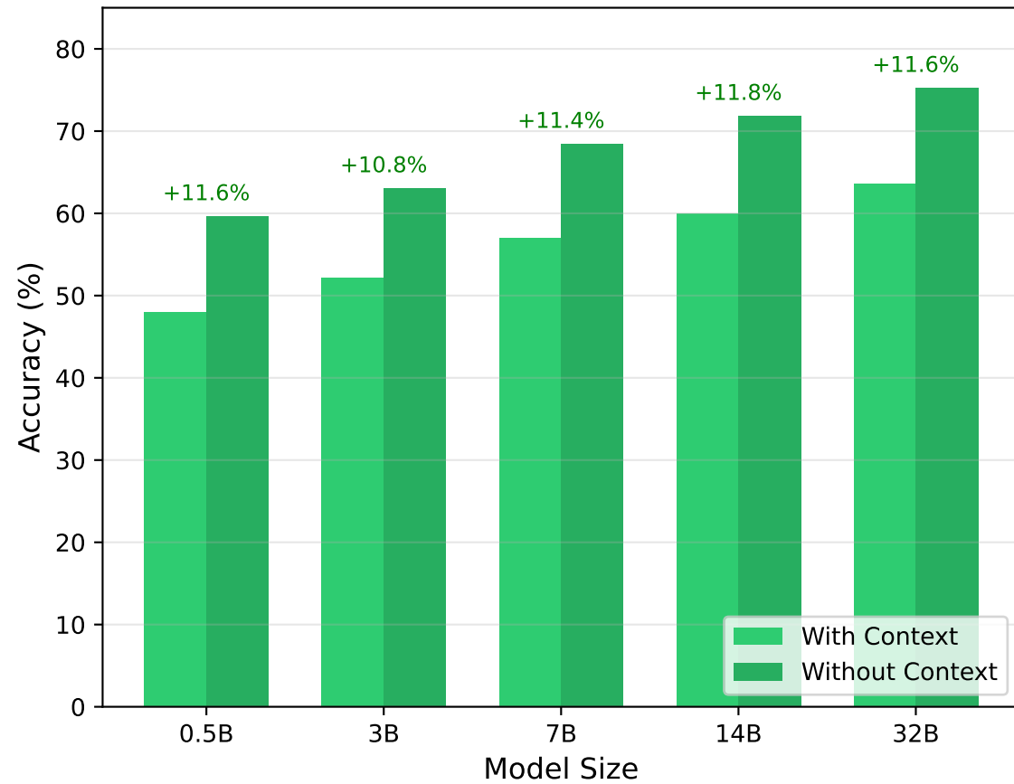
Gold Condition: Context as Noise
