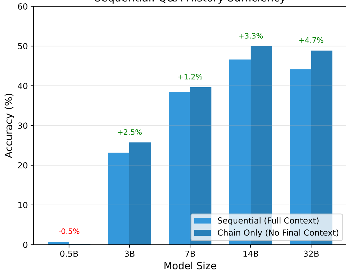
Sequential: Q&A History Sufficiency
