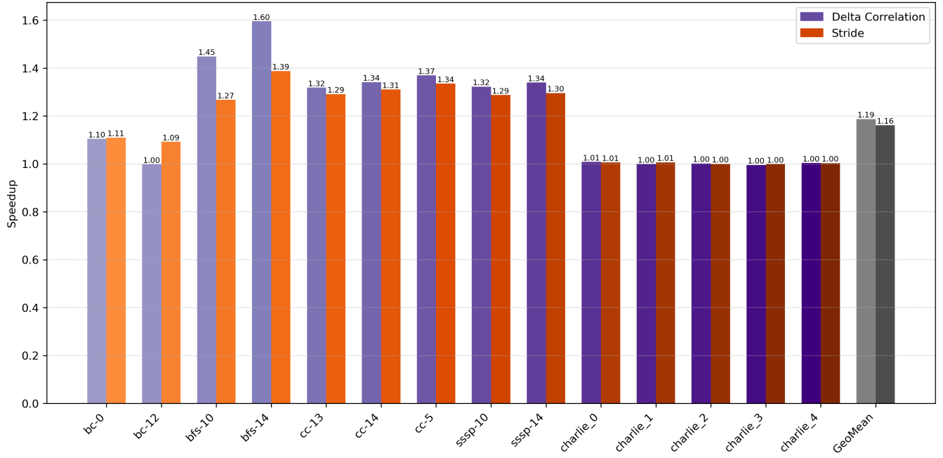
Figure 7: Delta correlation prefetcher and system-aware GHB-stride prefetcher speedup at limited bandwidth.
