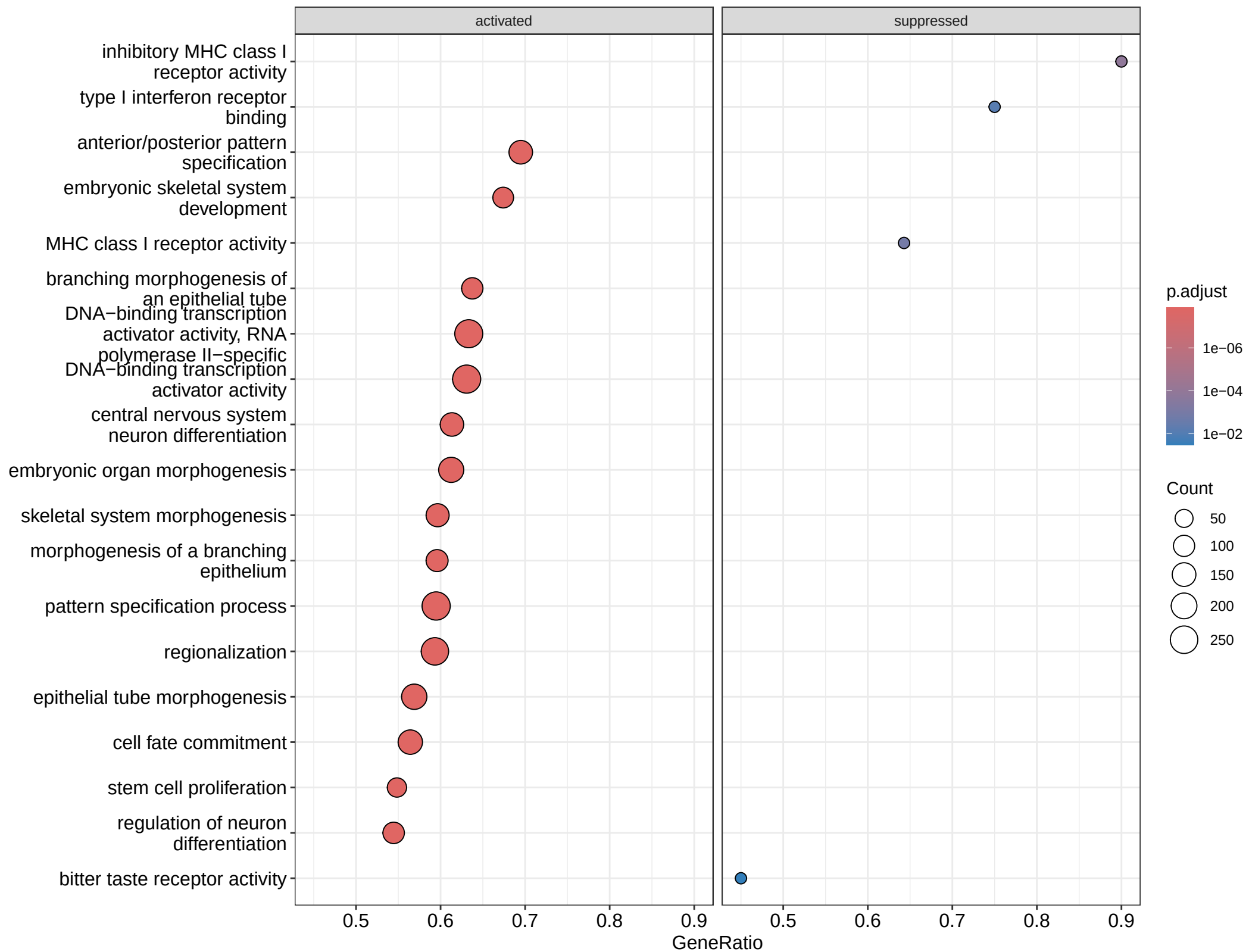
GO Enrichment: LNCAP vs PREC Methylation
