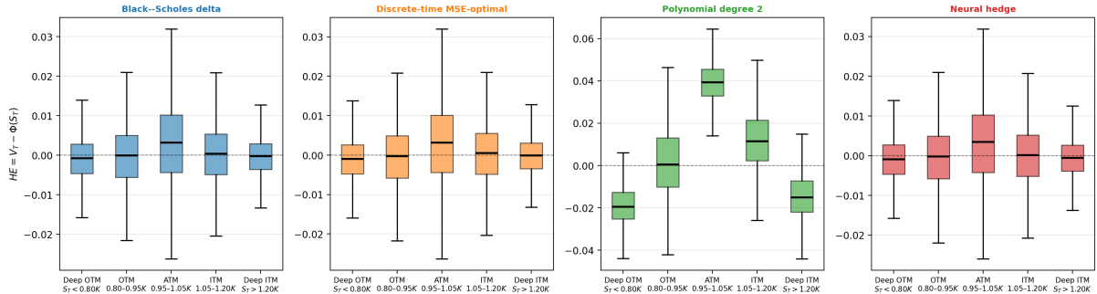
Distribution of hedge error HE by moneyness bucket Box = IQR, whiskers = 1.5 \times IQR, fliers suppressed for readability
