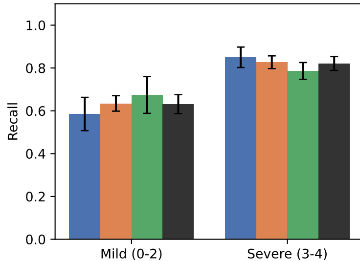
Recall
