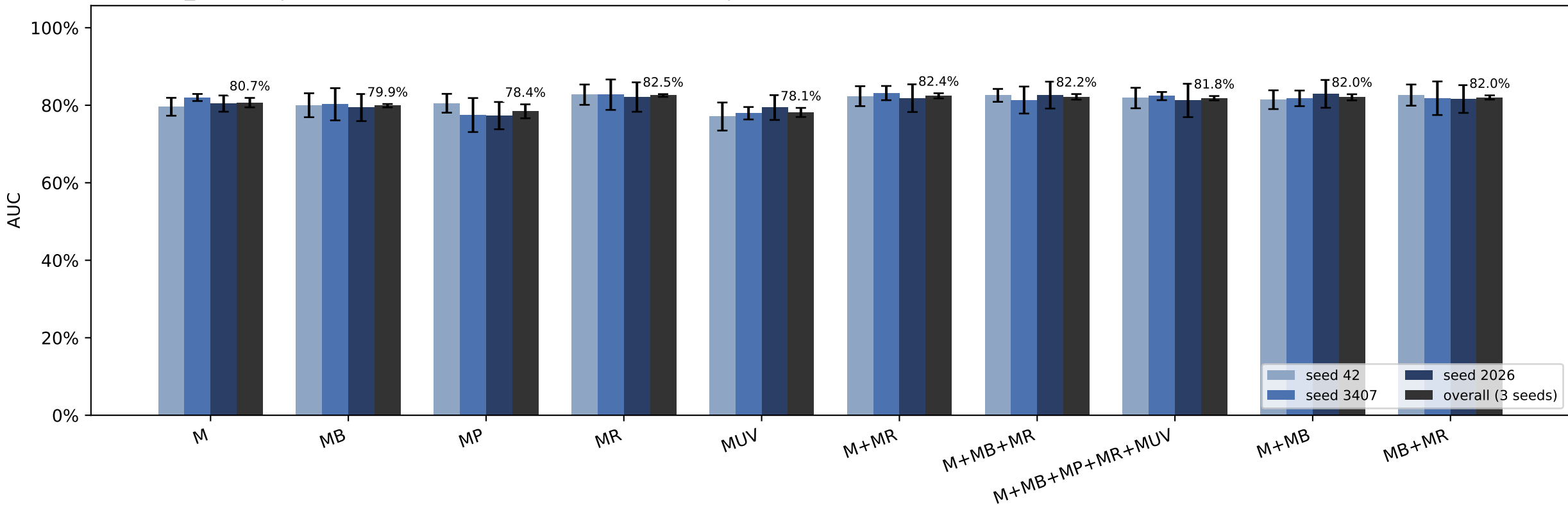
Step 03_I binary | White baseline vs multi-channel schemes | AUC (bar = mean over 5 folds; error bar = std; singles reused from Step 01/02)
