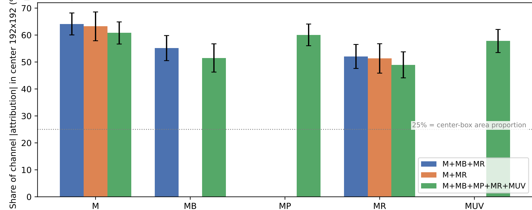
ep 04 | binary | DeepLIFT center-vs-periphery split (center box = middle 50% of each side; mean \pm std over
