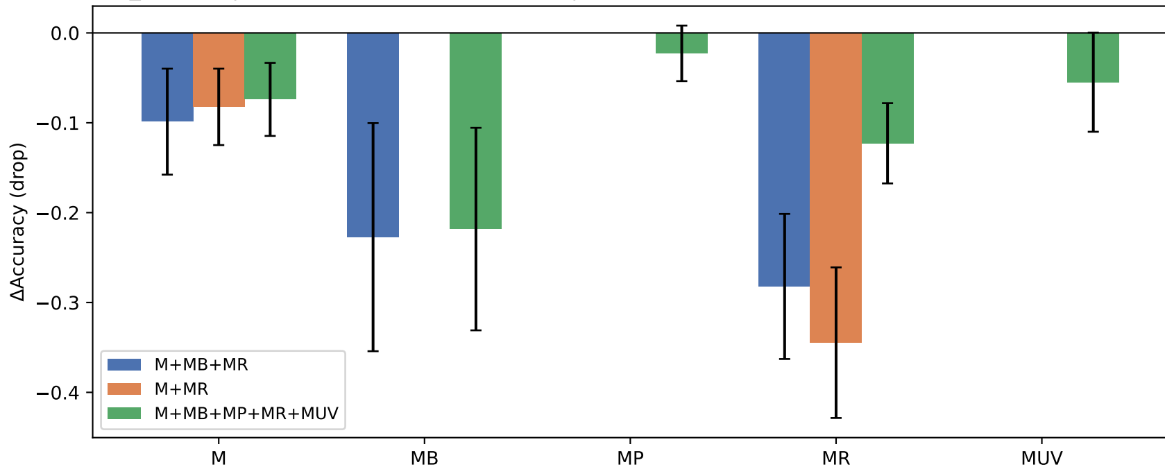
Step 04_I binary | channel perturbation impact | \Delta Accuracy (drop) (mean \pm std over 15 runs per scheme)
