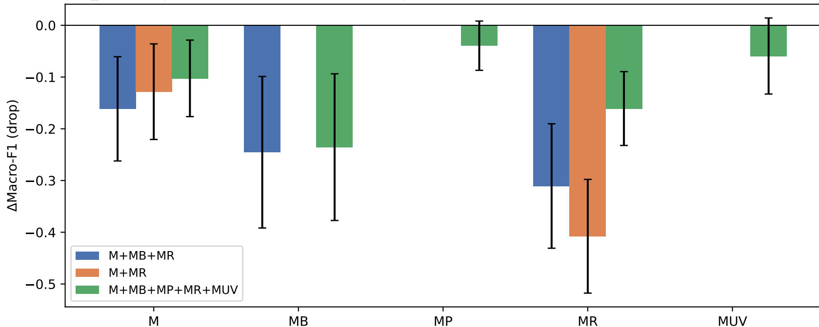
Step 04_I binary | channel perturbation impact | \Delta Macro-F1 (drop) (mean \pm std over 15 runs per scheme)
