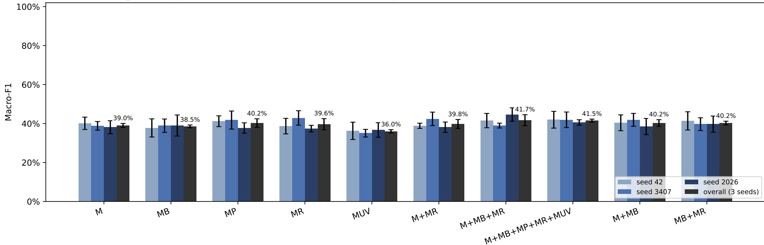
Step 06_1 5-class | White baseline vs multi-channel schemes | Macro-F1 (bar = mean over 5 folds; singles reused from Step 05)
