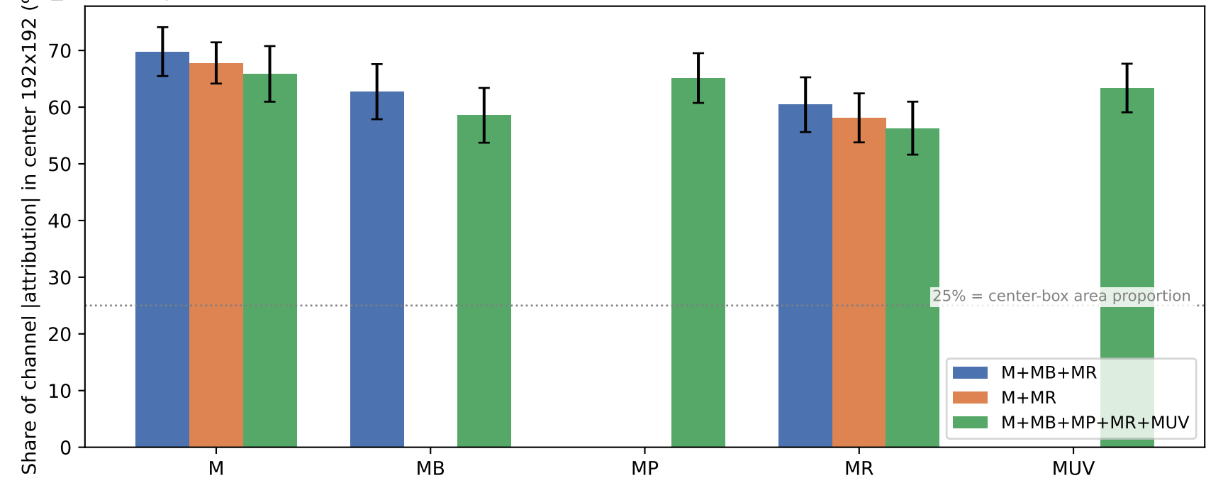
p17_1 5-class | DeepLIFT center-vs-periphery split (center box = middle 50% of each side; mean \pm std over
