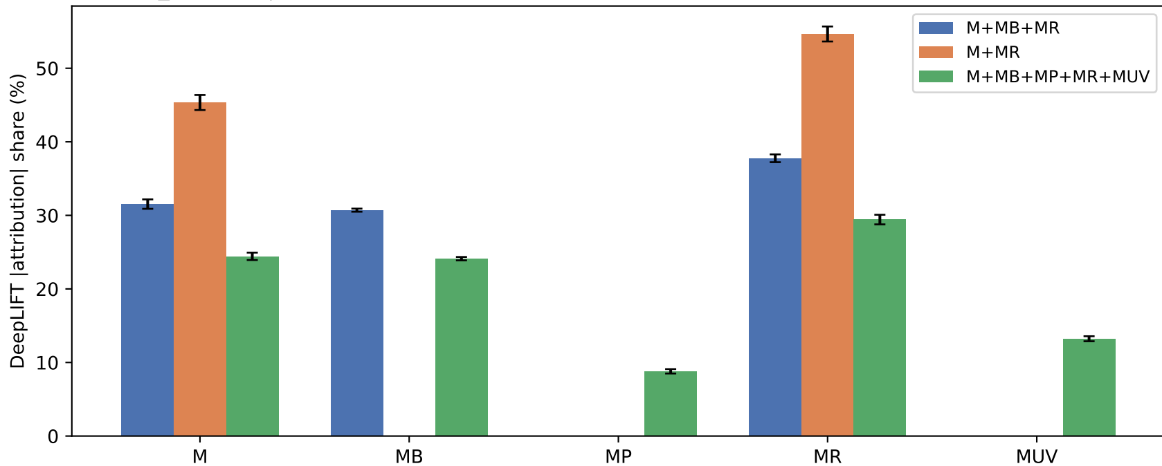
Step 07_I 5-class | per-channel DeepLIFT importance share (mean \pm std over 15 runs per scheme)
