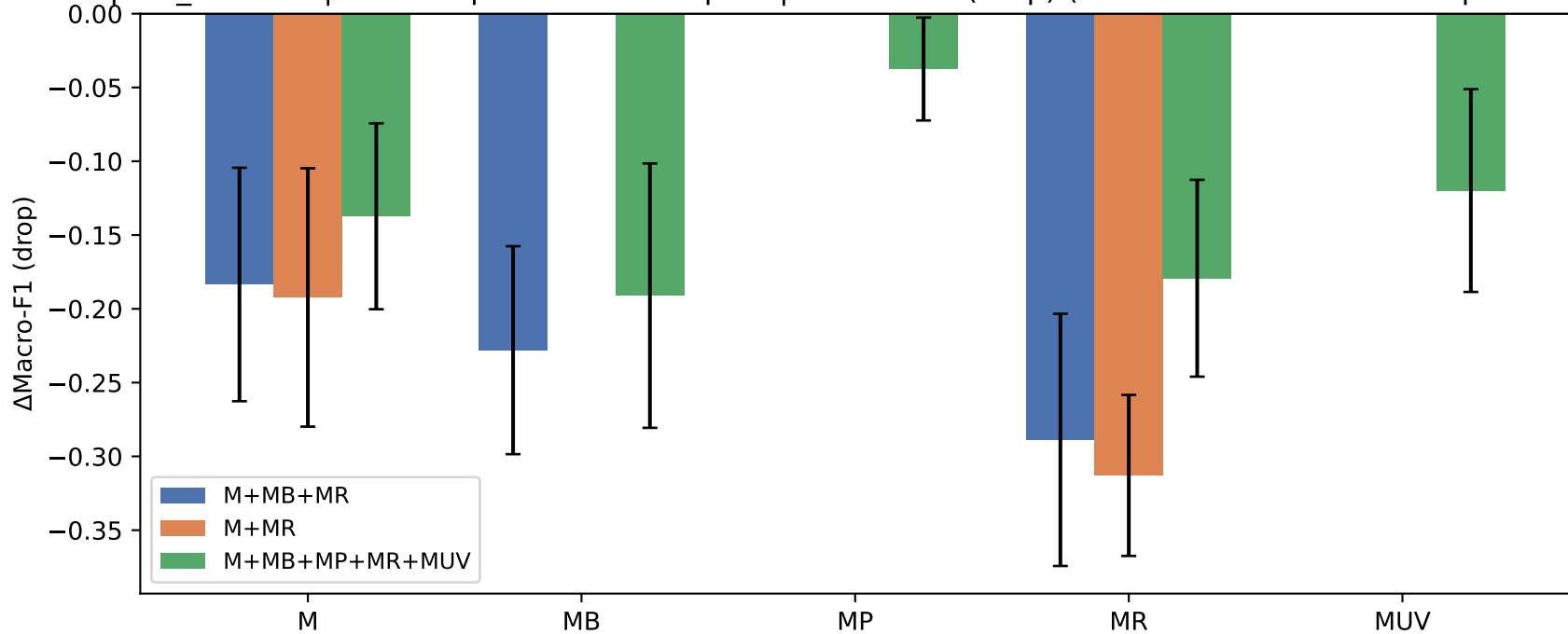
Step 07_1 5-class | channel perturbation impact | \Delta Macro-F1 (drop) (mean \pm std over 15 runs per scheduler)
