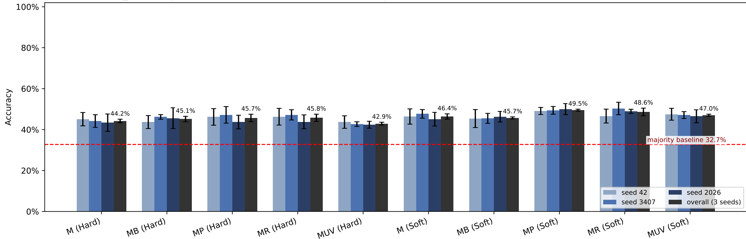
Step 08_1 5-class | White baseline vs multi-channel schemes | Accuracy (bar = mean over 5 folds; singles reused from Step 05)
