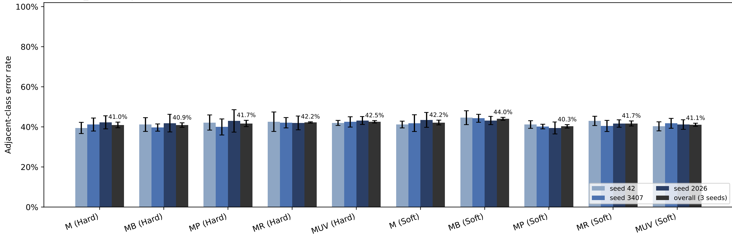
Step 08_1 5-class | White baseline vs multi-channel schemes | Adjacent-class error rate (bar = mean over 5 folds; singles reused from Step 05)
