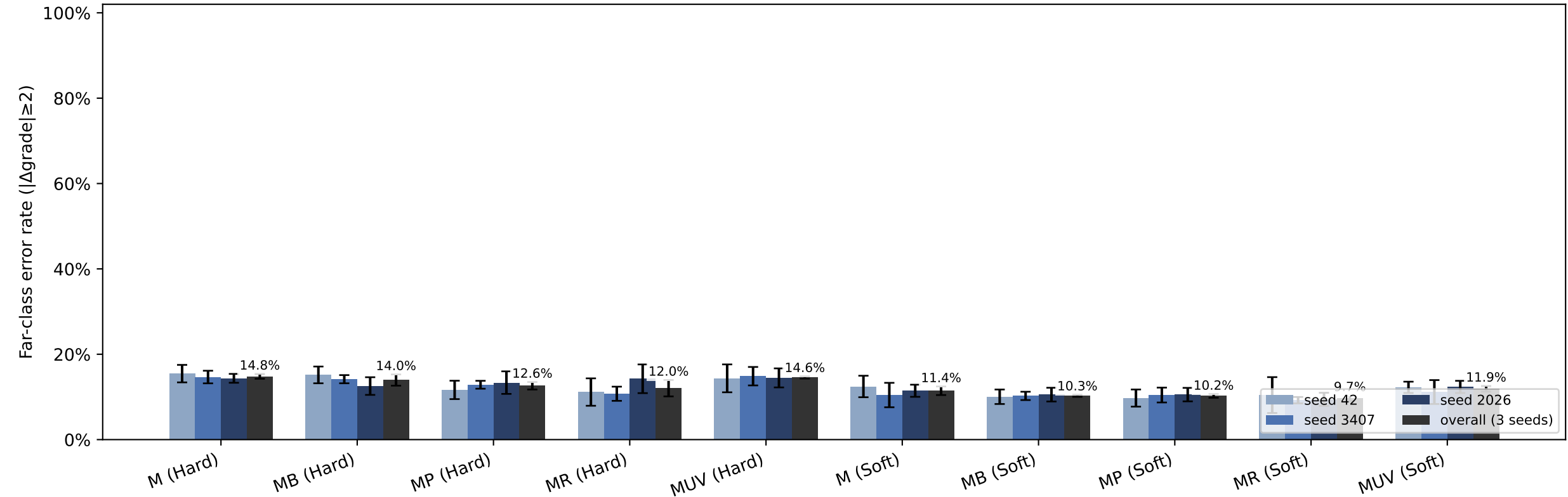
Step 08_I 5-class | White baseline vs multi-channel schemes | Far-class error rate ( |\Delta\text{grade}|\geq 2 ) (bar = mean over 5 folds; singles reused from Step 05)
