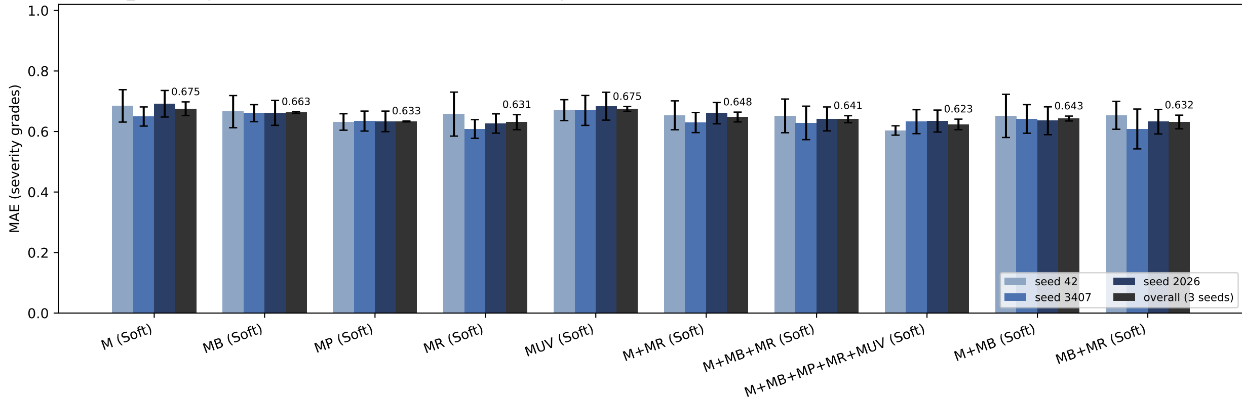
Step 09_1 5-class | White baseline vs multi-channel schemes | MAE (severity grades) (bar = mean over 5 folds; soft singles reused from Step 08)
