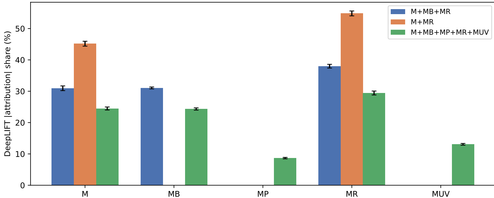
Step 10_I 5-class soft | per-channel DeepLIFT importance share (mean \pm std over 15 runs per scheme)
